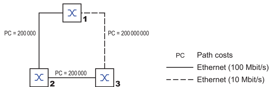
Figure 7: Path costs
