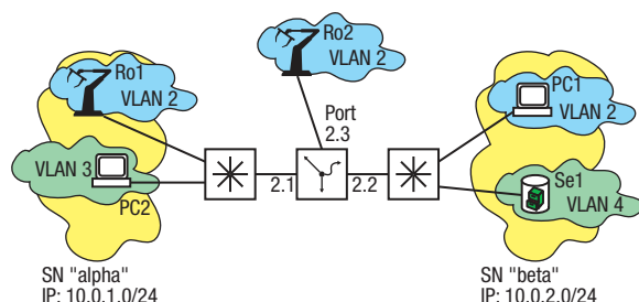
Figure 114: Application example of a protocol-based VLAN
