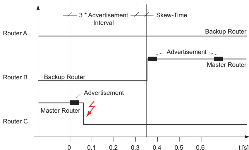
Figure 101: Master router <-> backup router failover times according to HiVRRP VRRP priority router A = 64 VRRP priority router B = 128 VRRP priority router C = 254
