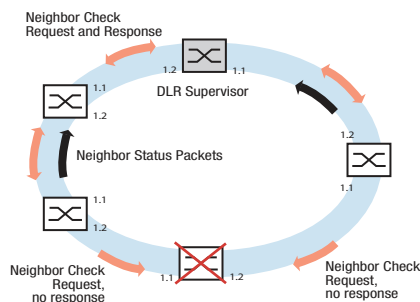
Figure 48: Neighbor Check process
