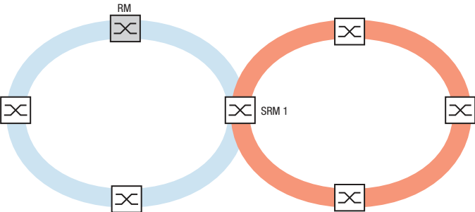
Figure 65: Special case: A Sub Ring Manager device manages both ends of a Sub Ring on different ports (Single Sub Ring Manager).
