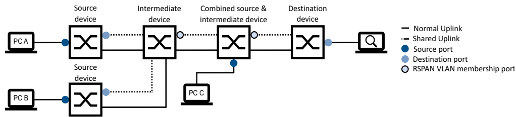
Figure 131: Example of a complex tree topology, without reflector ports (with separate uplinks)
