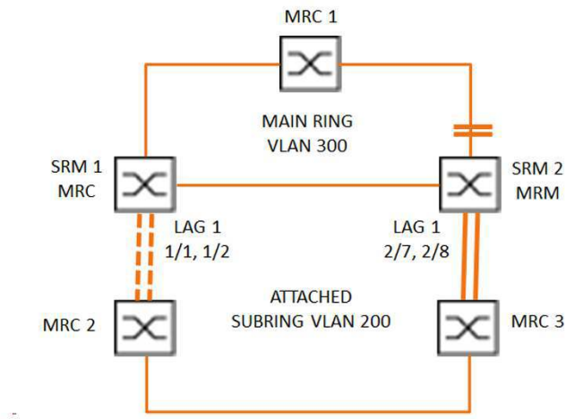
Figure 68: Sub Ring with Link Aggregation
