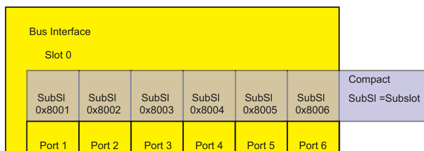
Figure 146: Compact device
