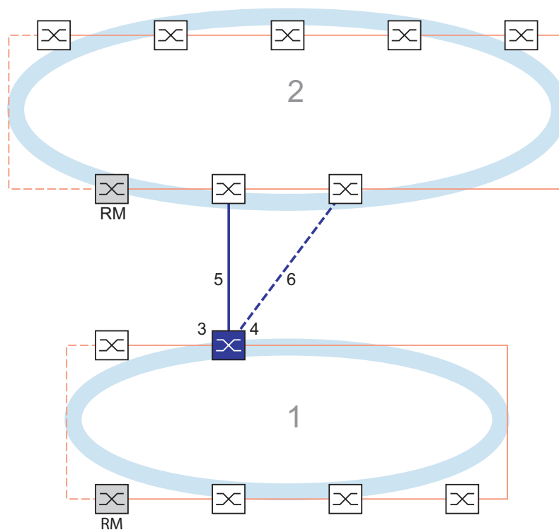
Figure 76: Example of 1-Switch coupling 1: Ring 2: Backbone 3: Partner coupling port 4: Coupling port 5: Main line 6: Redundant line
