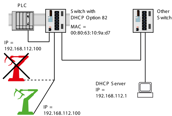
Figure 166: Application example of using Option 82
