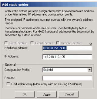
Figure 159:Entries for static addresses
