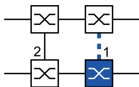
Figure 80: 2-Switch coupling, Stand-by device 1: Coupling port 2: Partner coupling port
