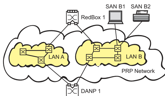
Figure 41: Parallel Redundancy Protocol Network
