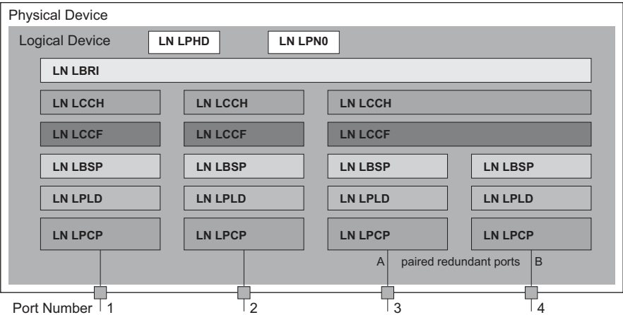
Figure 141: Bridge model based on Technical Report IEC 61850 90-4
