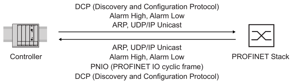
Figure 145: Communication between the Controller and the device
