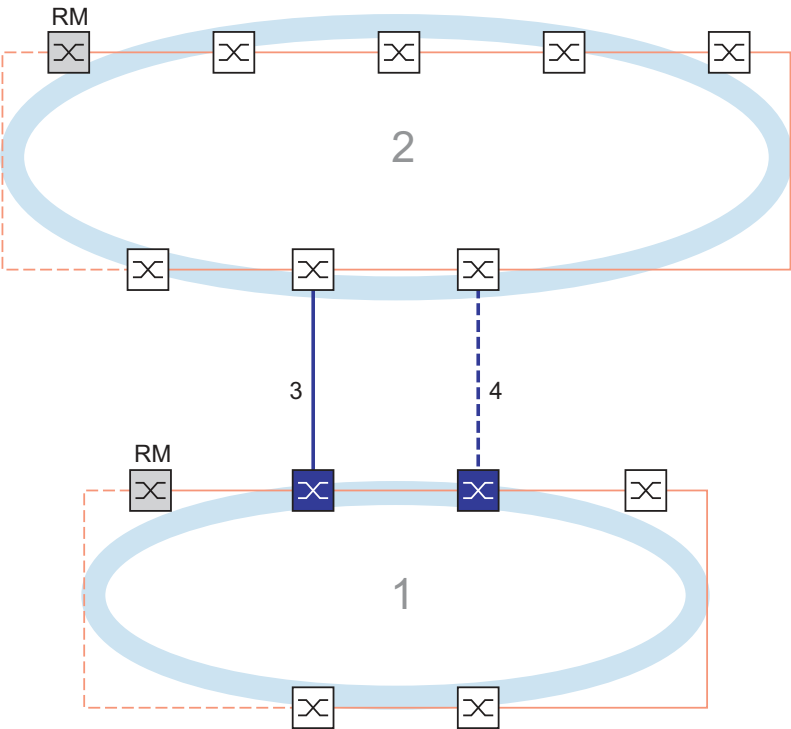
Figure 78: Example of 2-Switch coupling 1: Ring 2: Backbone 3: Main line 4: Redundant line
