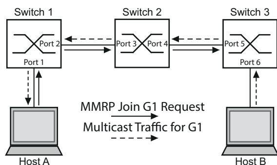
Figure 138: MMRP Network for MAC address Registration
