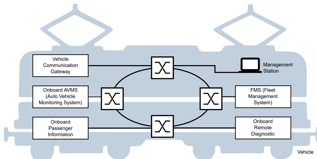
Figure 150: Example for ITxPT Module Inventory
