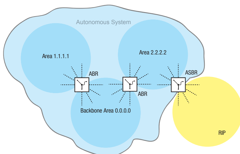
Figure 108: Autonomous System
