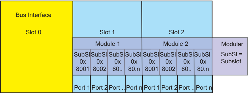
Figure 147: Modular device
