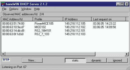
Figure 160:DHCP server with entries
