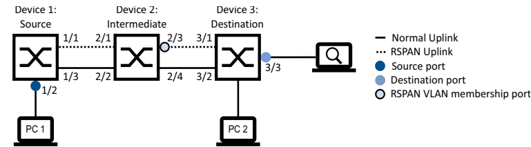
Figure 135: RSPAN in a line topology, without a reflector port (with separate uplinks)
