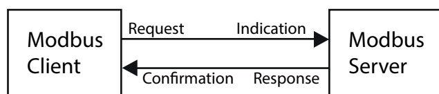
Figure 142: Client/Server Modbus TCP/IP Mode
