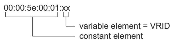
Figure 99: Virtual MAC address
