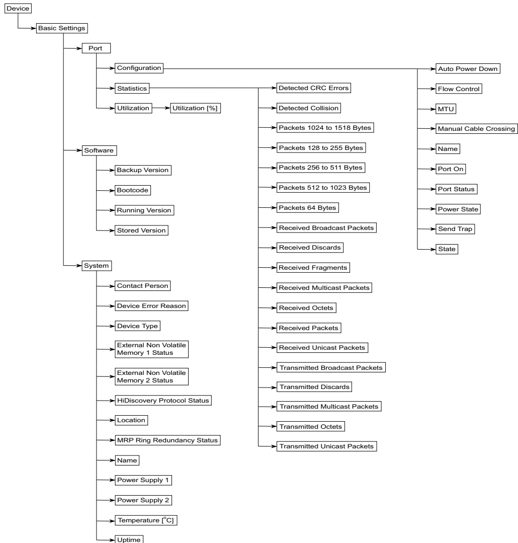
Figure 149: OPC UA information model
