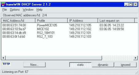
Figure 154:DHCP server with entries
