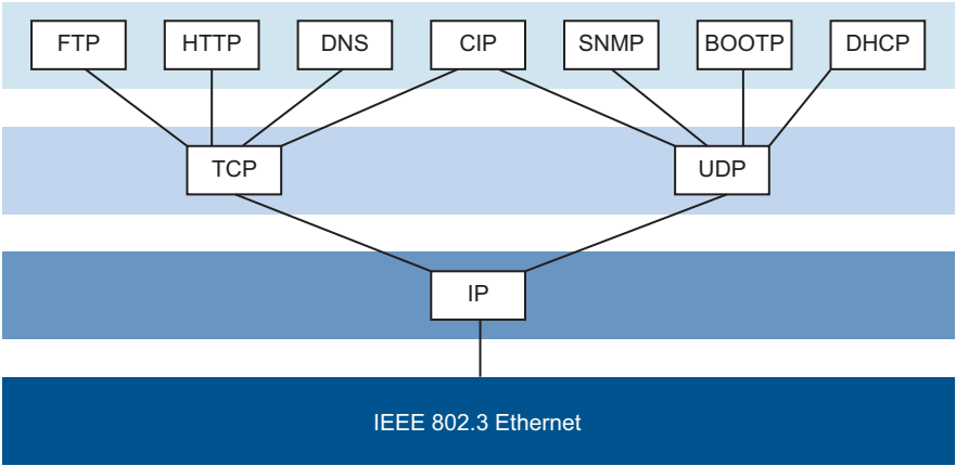
Figure 138: IEEE 802.3 EtherNet/IP
