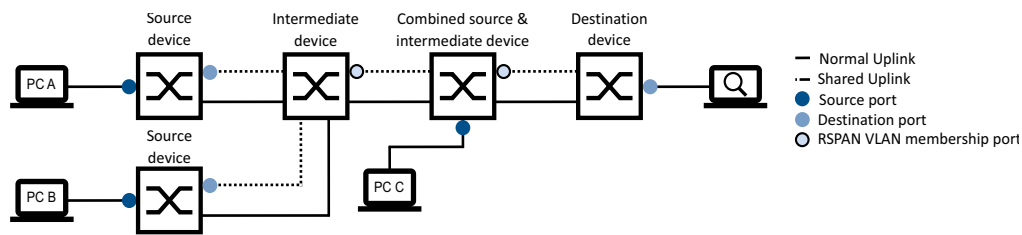
Figure 124: Example of a complex tree topology, without reflector ports (with separate uplinks)
