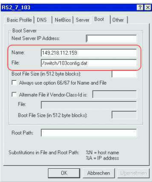
Figure 149: Configuration file on the tftp server
