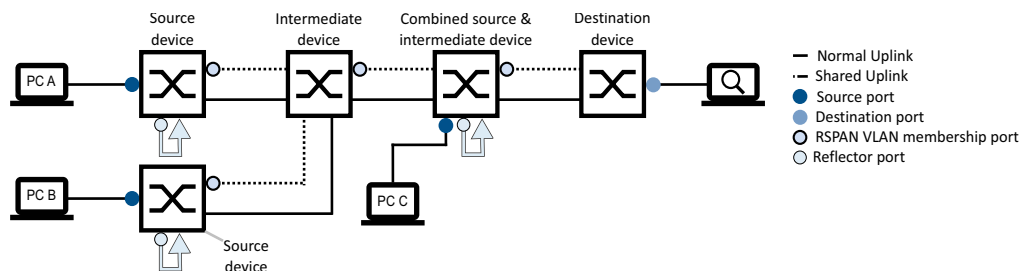
Figure 123: Example of a complex tree topology, using reflector ports (with separate uplinks)
