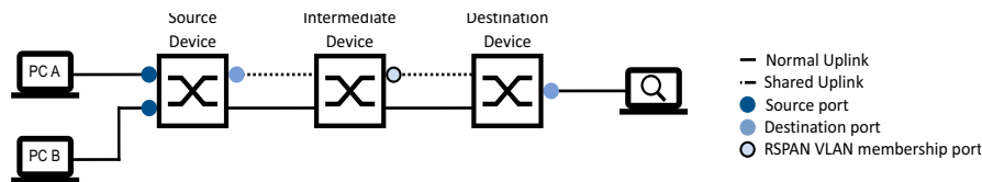
Figure 122: Example of a line topology, without a reflector port (with separate uplinks)
