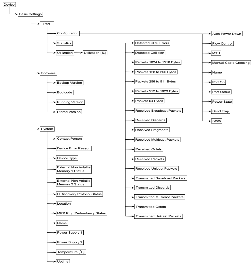
Figure 143: OPC UA information model
