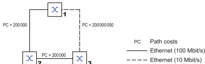
Figure 44: Path costs
