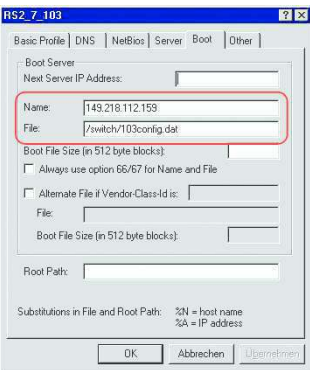
Figure 111: Configuration file on the tftp server
