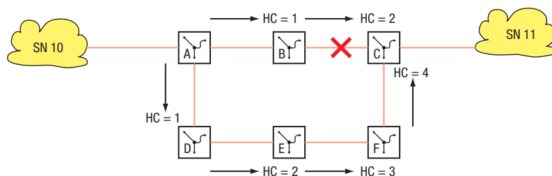
Abb. 100: Hop-Count
