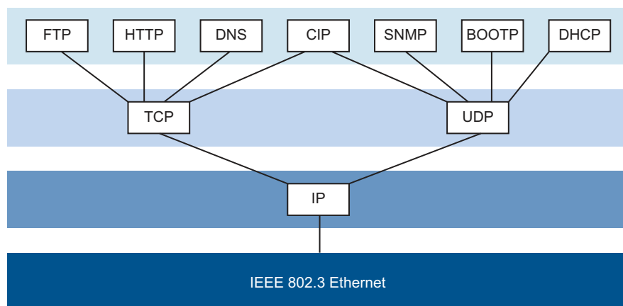
Abb. 135: IEEE802.3 EtherNet/IP
