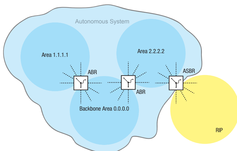
Abb. 102: Autonomes System
