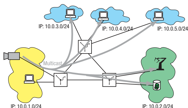
Abb. 111: Multicast Flooding
