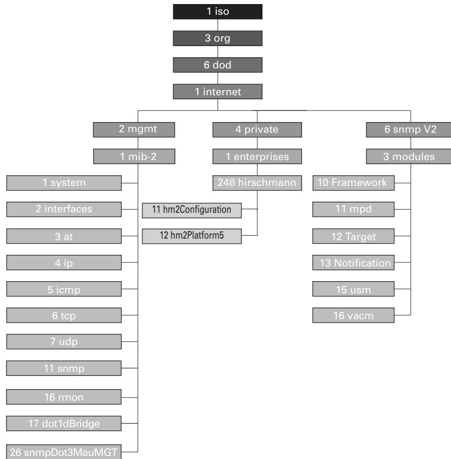
Figure 164: Tree structure of the Hirschmann MIB
