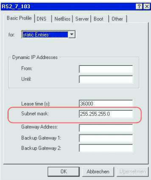
Figure 149: Netmask in the configuration profile
