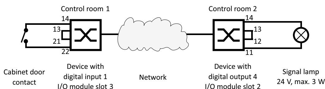
Figure 132: Mirroring an I/O signal over the network
