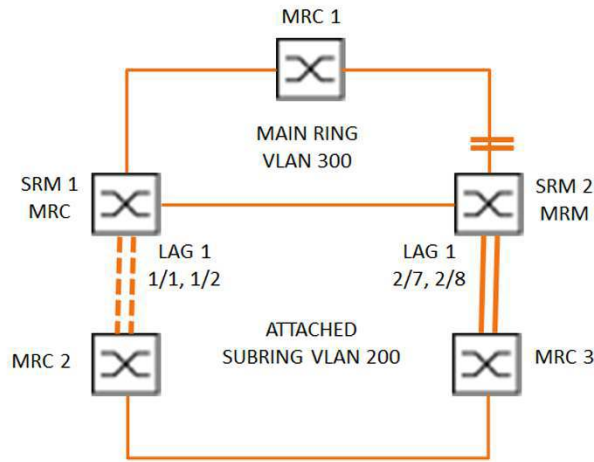
Figure 62: Sub Ring with Link Aggregation
