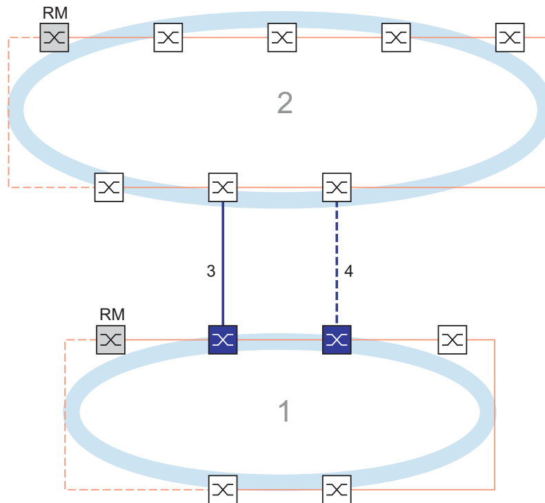
Figure 64: Example of 2-Switch coupling
