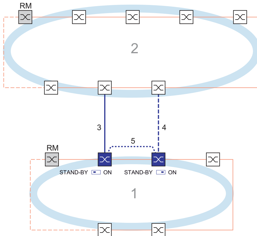
Figure 75: Example of 2-Switch coupling with control line
