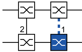
Figure 74: 2-Switch coupling, Stand-by device
