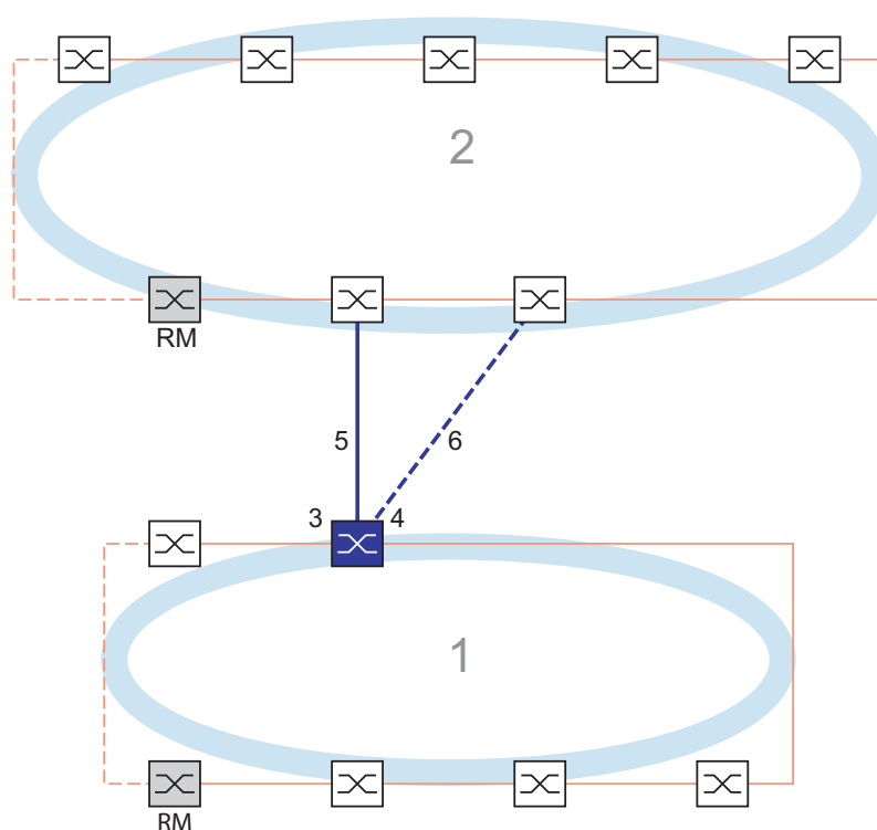
Figure 70: Example of 1-Switch coupling 1: Ring 2: Backbone 3: Partner coupling port 4: Coupling port 5: Main line 6: Redundant line
