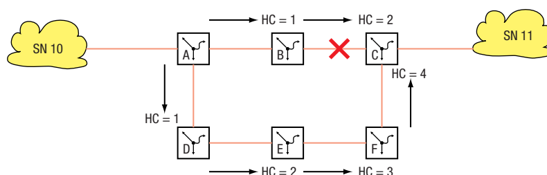
Abb. 97: Hop-Count
