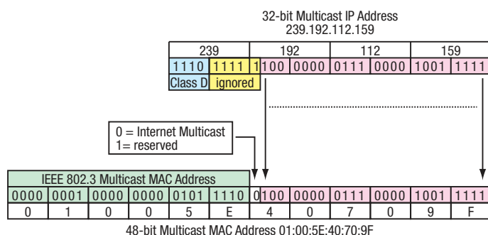
Figure 107: Conversion of the IP address to the MAC address
