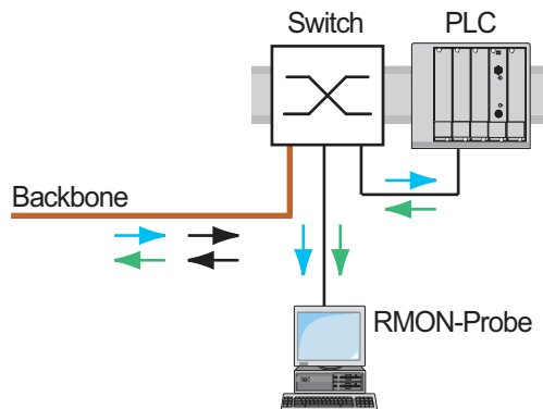
Figure 117: Application example of a port-mirroring setup
