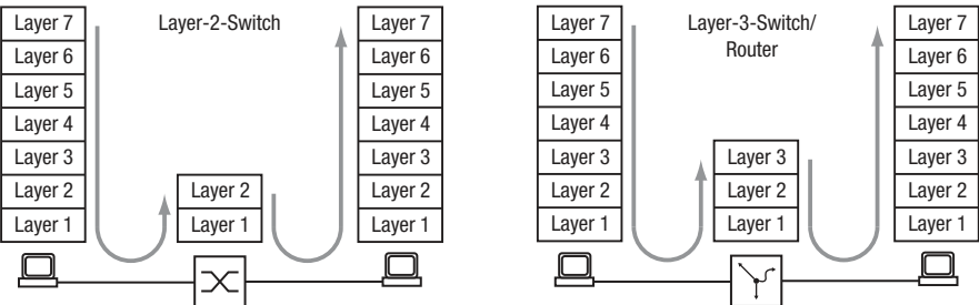
Figure 78: Data Transport by a Switch and a Router in the OSI Reference Model's Layers
