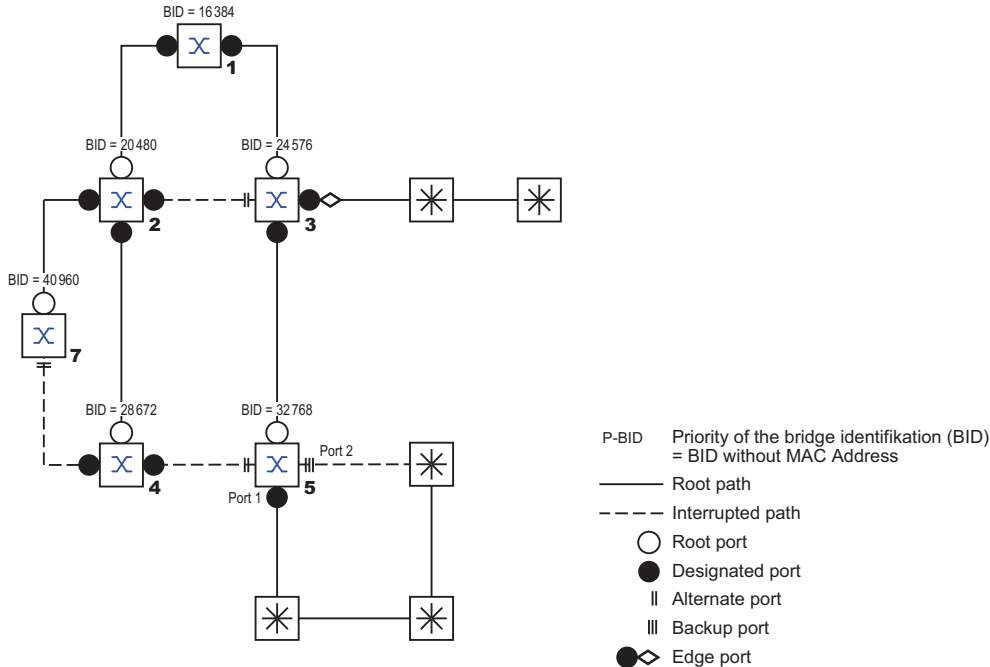
Figure 51: Port role assignment
