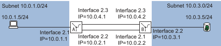
Figure 88: Redundant static route
