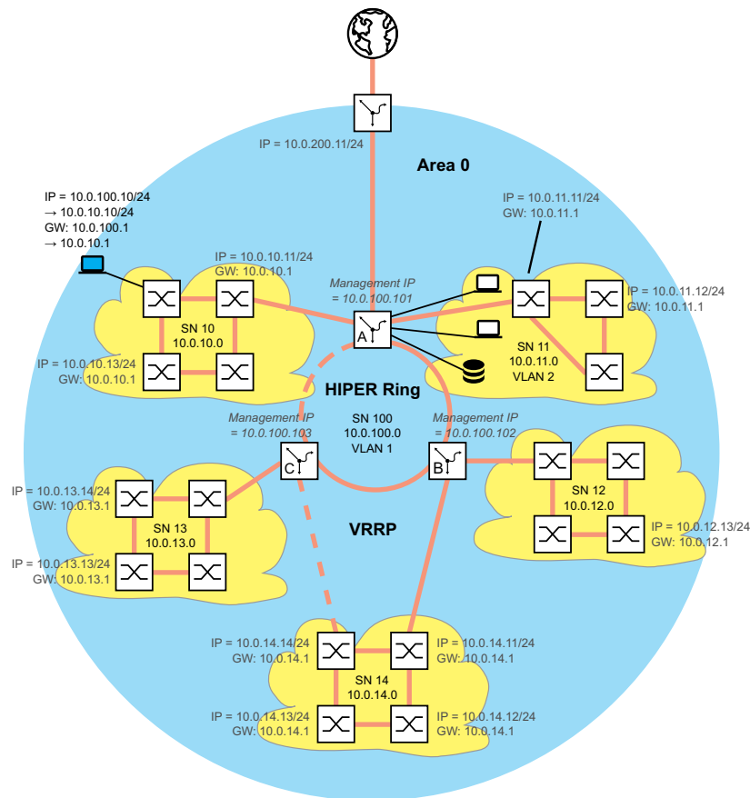
Figure 109: Network plan with management IP addresses
