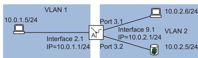
Figure 86: VLAN-based router interface
