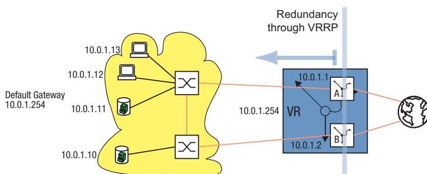
Figure 89: Illustration of the virtual router
