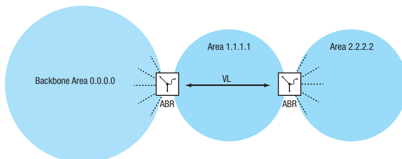
Figure 101: Linking a remote area to the backbone area using a virtual link (VL)
