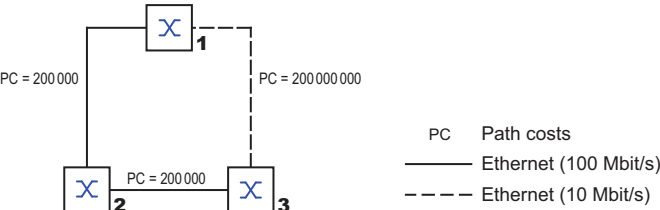
Figure 43: Path costs
