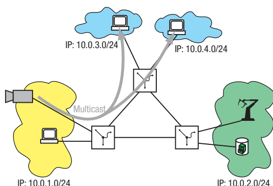
Figure 106: Example of a multicast application
