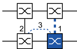
Figure 75: 2-Switch coupling with Control Line, Stand-by device 1: Coupling port 2: Partner coupling port 3: Control line
