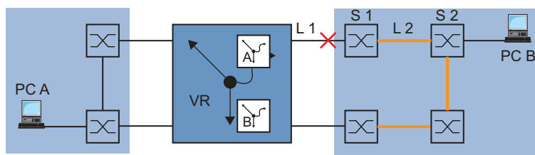
Figure 111: Monitoring a line with interface tracking
