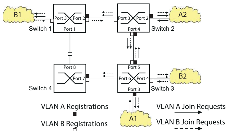
Figure 131: MVRP Example Network for VLAN Registration
