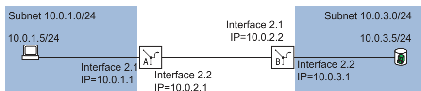
Figure 87: Static Routing
