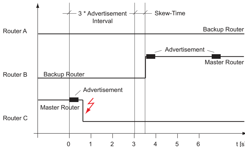
Figure 91: Master router <-> backup router failover times according to RFC 2338 VRRP priority router A = 64 VRRP priority router B = 128 VRRP priority router C = 254
