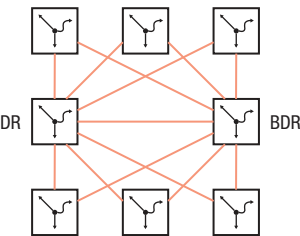
Figure 103: LSA distribution with designated router and backup designated router
