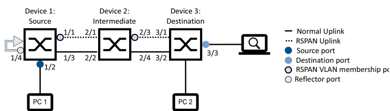
Figure 124: RSPAN in a line topology, using a reflector port (with separate uplinks)
