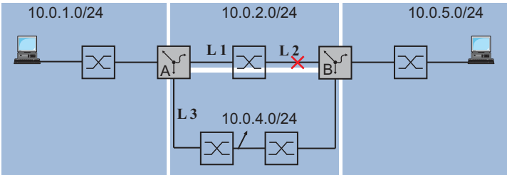
Figure 114: Example of static route tracking
