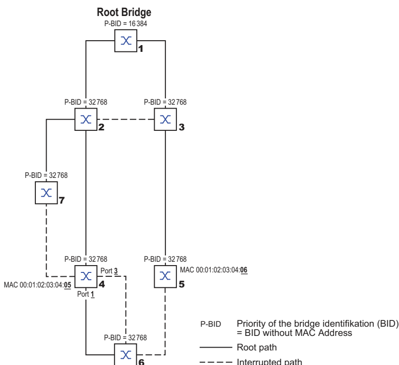
Figure 48: Example of a network plan for determining the root path
