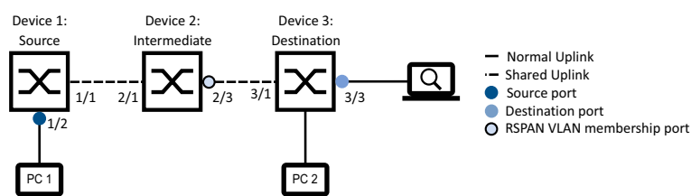
Figure 127: RSPAN in a line topology, without a reflector port (with shared uplinks)
