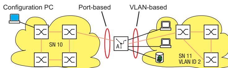
Figure 84: Static routes: Example of connecting two production cells
