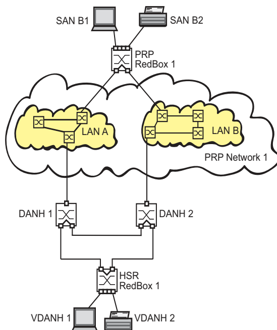
Figure 41: Connecting a PRP network to an HSR network
