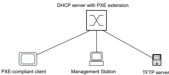
Figure 128: Simple structure of a Preboot eXecution Environment (PXE) setup
