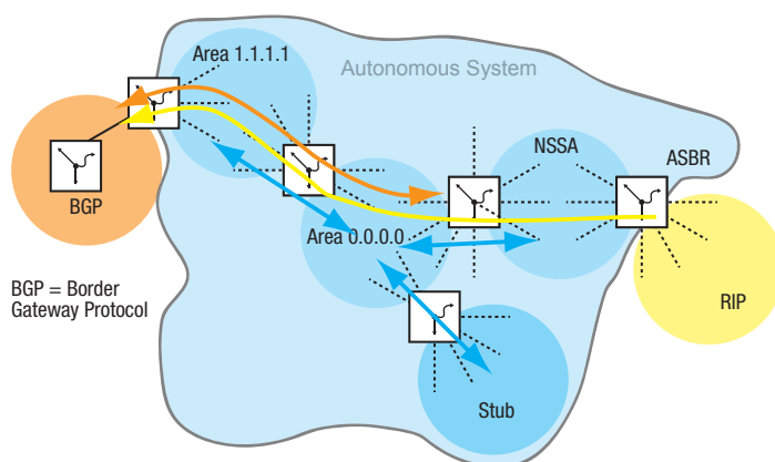
Figure 100: LSA distribution into the area types
