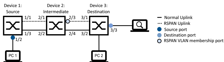
Figure 126: RSPAN in a line topology, without a reflector port (with separate uplinks)
