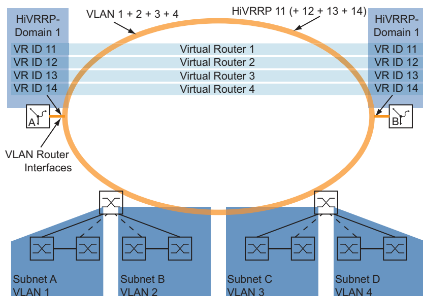
Figure 93: Example of how a HiVRRP domain is used
