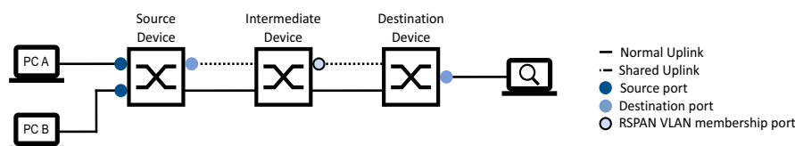
Figure 120: Example of a line topology, without a reflector port (with separate uplinks)
