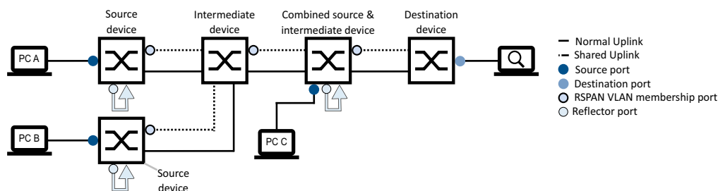
Figure 121: Example of a complex tree topology, using reflector ports (with separate uplinks)
