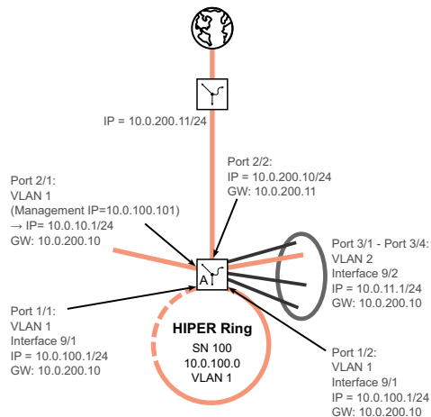
Figure 110: IP parameters for Layer 3 device A
