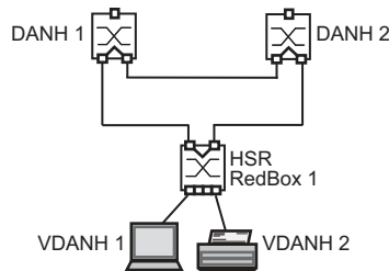
Figure 40: Connecting a VDANH to an HSR network
