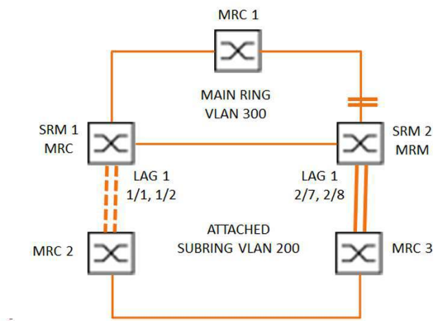
Figure 60: Sub Ring with Link Aggregation
