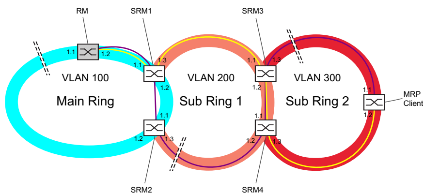
Figure 59: Example of a cascaded Sub Ring structure Blue circle = Main ring members in VLAN 100 Orange circle = Sub Ring members in VLAN 200 Red circle = Sub Ring members in VLAN 300 Yellow line = Main network link Purple line = Redundant network link Dashed black lines = Blocked network link SRM1 = Sub Ring Manager for Sub Ring 1 and MRP client for the Main Ring SRM2 = Redundant Sub Ring Manager for Sub Ring 1 and MRP client for the Main Ring SRM3 = Redundant Sub Ring Manager for Sub Ring 2 and MRP client for Sub Ring 1 SRM4 = Sub Ring Manager for Sub Ring 2 and MRP client for Sub Ring 1 MRP Client = MRP Client participating in Sub Ring 2 RM = Ring Manager
