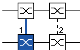
Figure 71: 2-Switch coupling, Primary device
