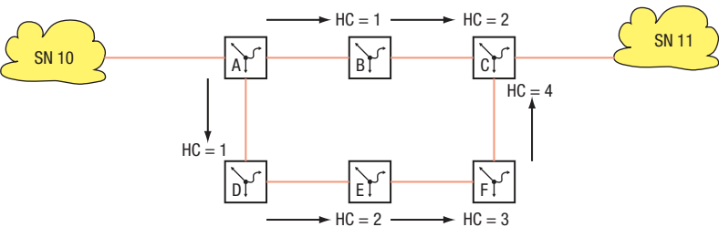
Figure 96: Counting Hops
