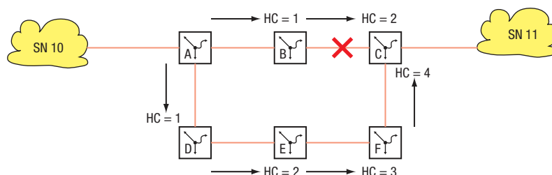
Abb. 99: Hop-Count
