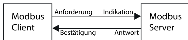
Abb. 52: Modbus TCP/IP Client/Server-Modus
