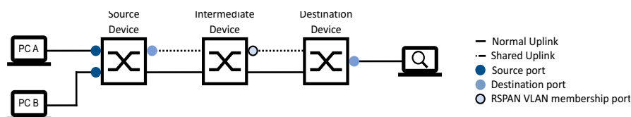
Figure 84: Example of a line topology, without a reflector port (with separate uplinks)
