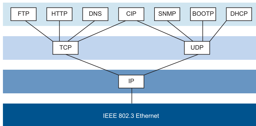
Figure 137: IEEE 802.3 EtherNet/IP
