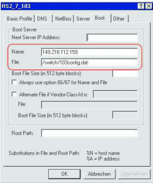
Figure 106: Configuration file on the tftp server
