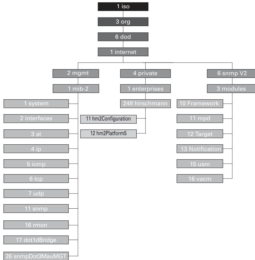
Figure 118: Tree structure of the Hirschmann MIB
