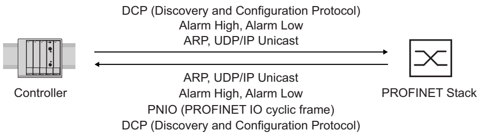
Figure 98: Communication between the Controller and the device
