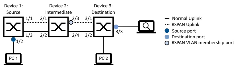
Figure 86: RSPAN in a line topology, without a reflector port (with separate uplinks)
