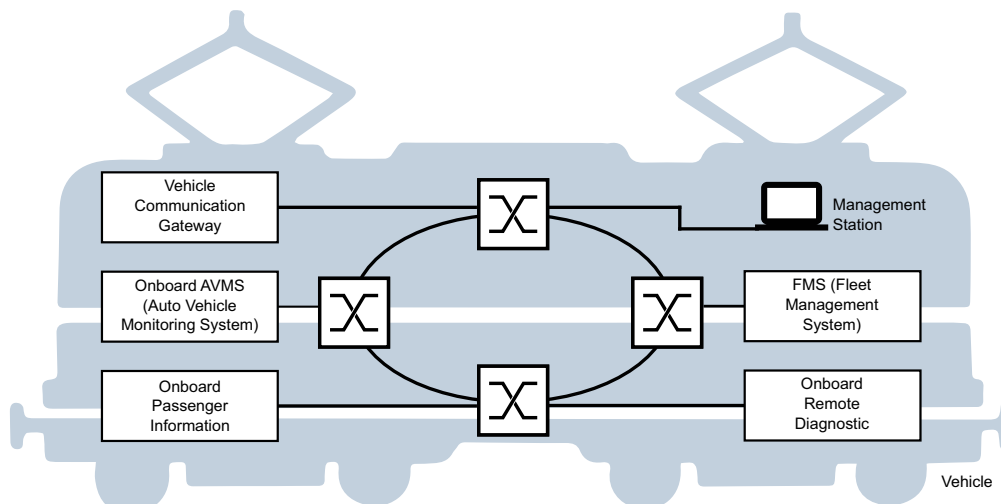
Figure 97: Example for ITxPT Module Inventory
