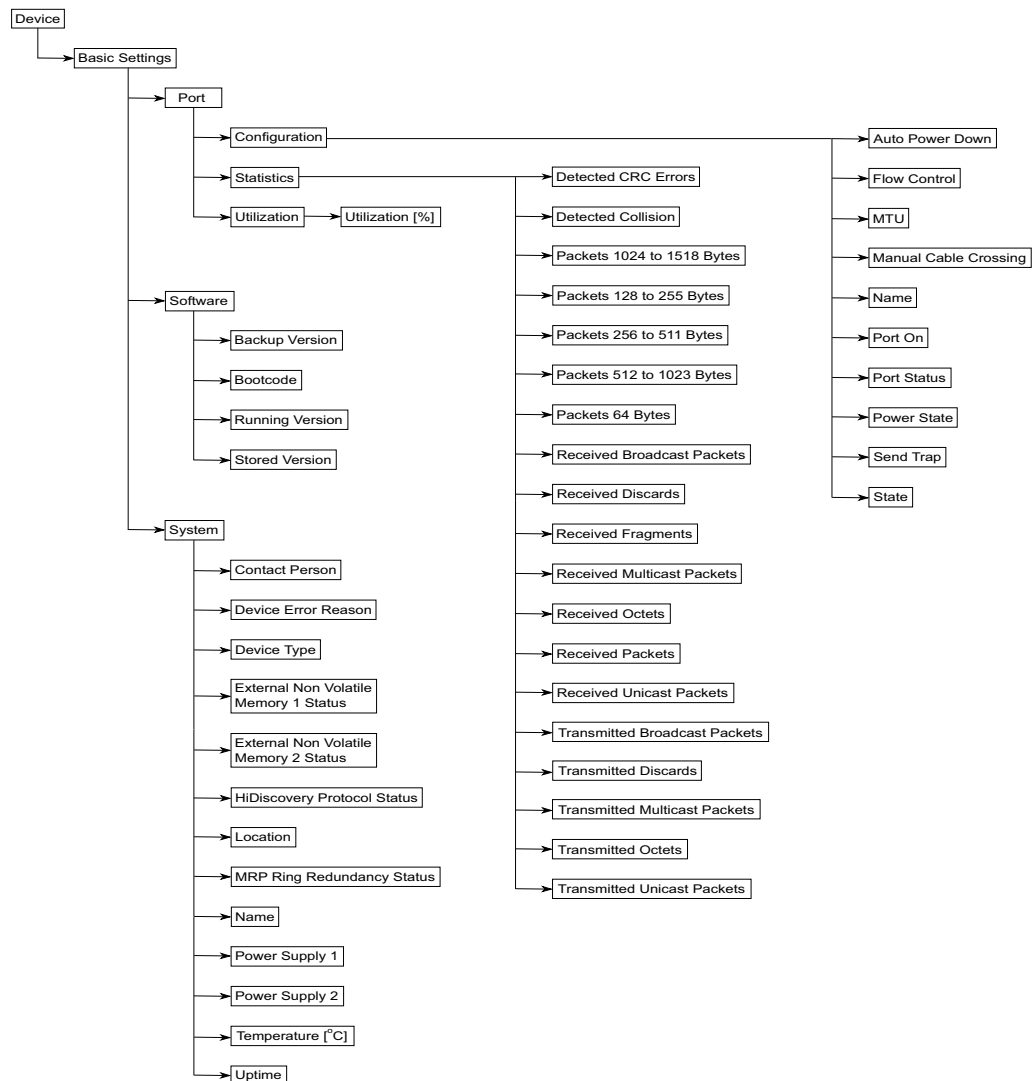
Figure 103: OPC UA information model
