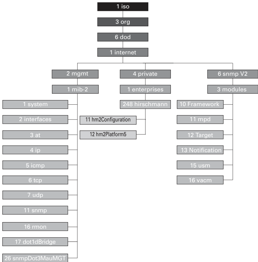
Figure 123: Tree structure of the Hirschmann MIB
