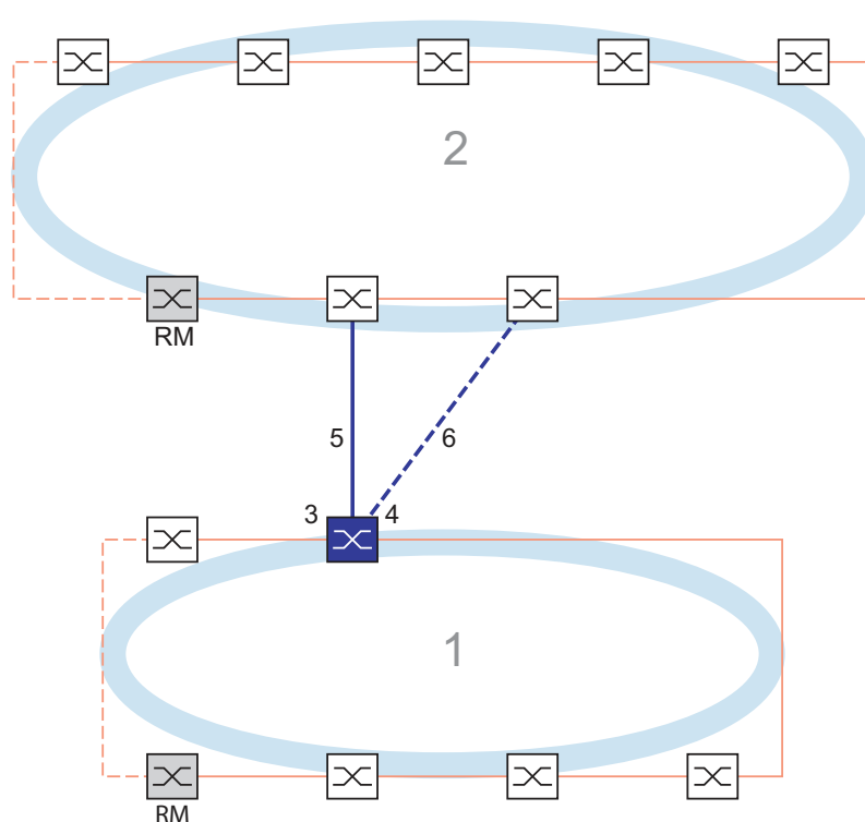
Figure 69: Example of 1-Switch coupling 1: Ring 2: Backbone 3: Partner coupling port 4: Coupling port 5: Main line 6: Redundant line
