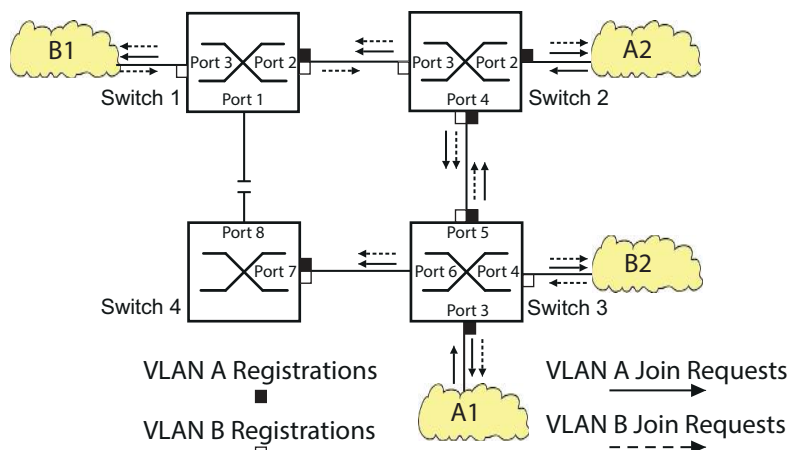
Figure 94: MVRP Example Network for VLAN Registration
