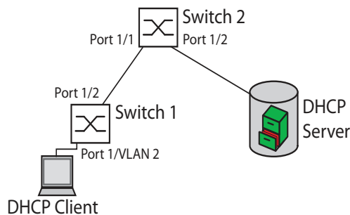
Figure 92: DHCP Layer 2 Example Network
