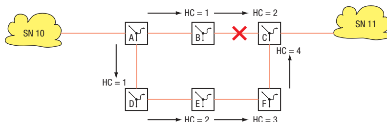
Abb. 104: Hop-Count
