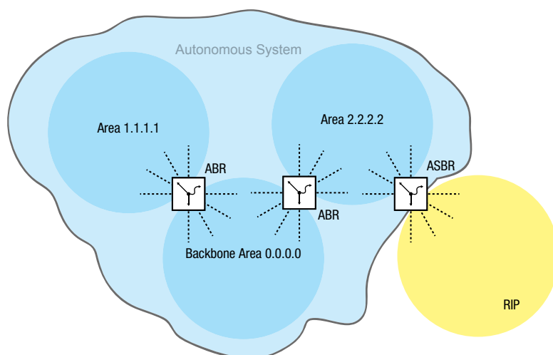
Abb. 53: Autonomes System
