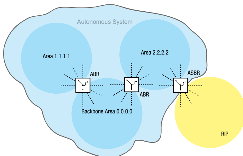
Abb. 93: Autonomes System
