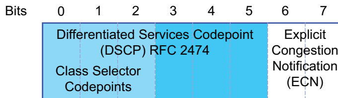
Abb. 22: Differentiated-Services-Feld im IP-Header
