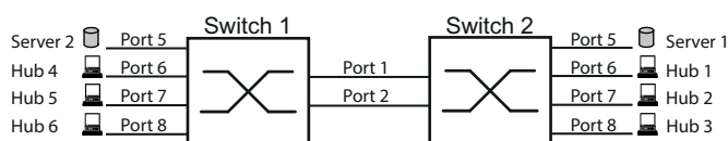
Abb. 45: Link Aggregation Switch-zu-Switch-Netz
