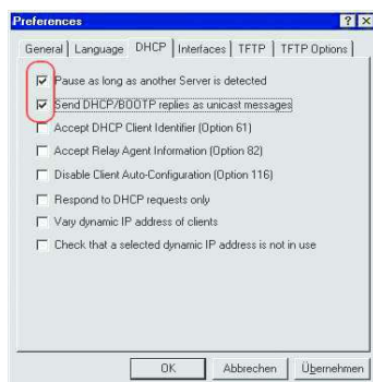
Figure 96: DHCP setting
