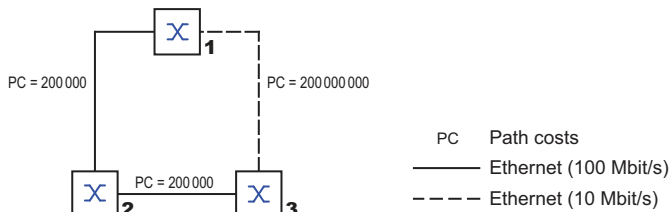
Figure 40: Path costs
