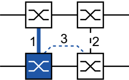
Figure 63: 2-Switch coupling with Control Line, Primary device 1: Coupling port 2: Partner coupling port 3: Control line
