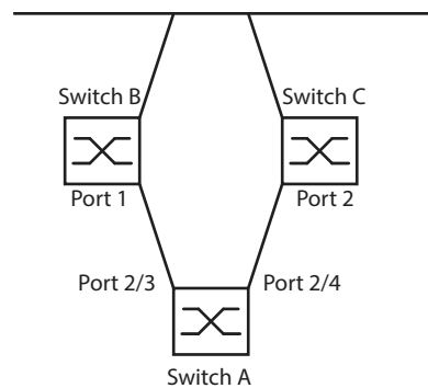
Figure 53: Link Backup example network
