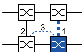
Figure 67: 2-Switch coupling with Control Line, Stand-by device
