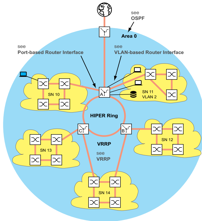
Figure 108: Network plan
