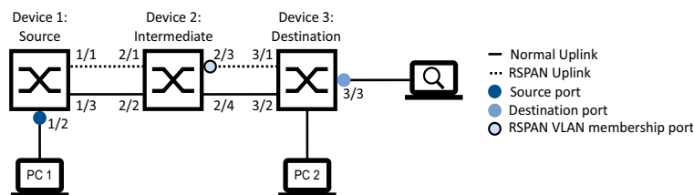
Figure 126: RSPAN in a line topology, without a reflector port (with separate uplinks)
