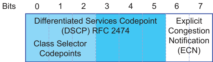
Figure 24: Differentiated Services field in the IP header
