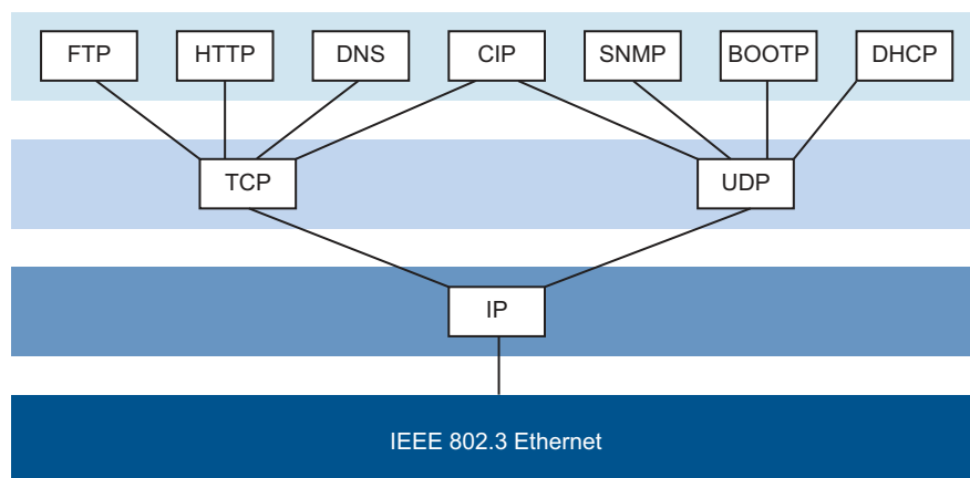
Figure 134: IEEE 802.3 EtherNet/IP
