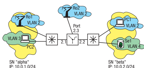
Figure 105: Application example of a protocol-based VLAN
