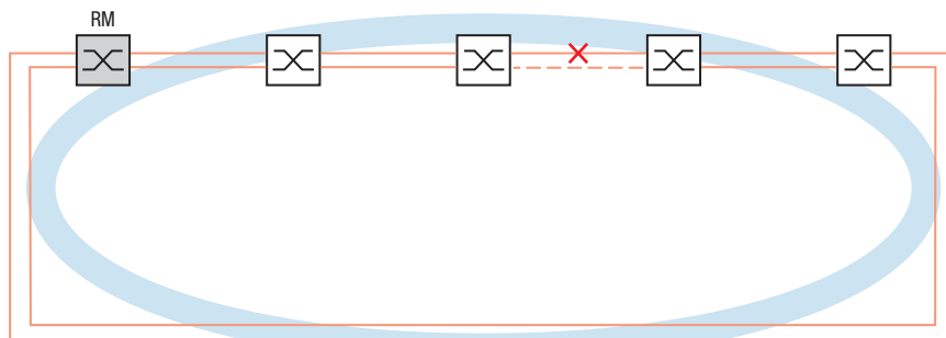
Figure 40: Interruption of a link in an MRP Ring
