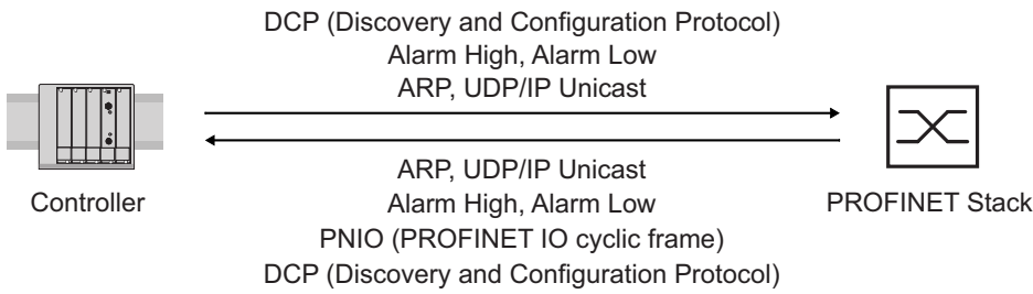
Figure 135: Communication between the Controller and the device
