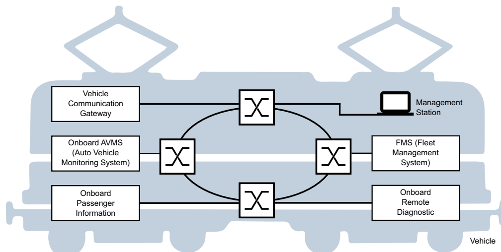
Figure 140: Example for ITxPT Module Inventory
