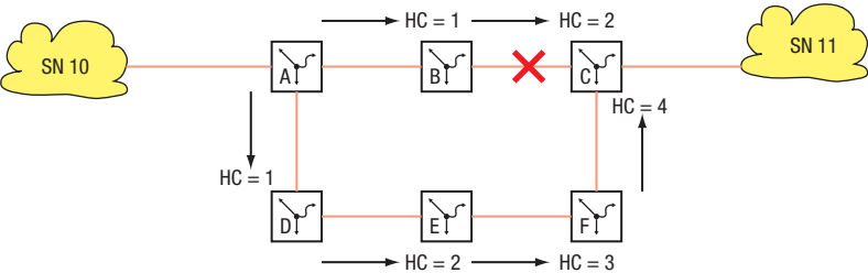
Figure 97: Hop count
