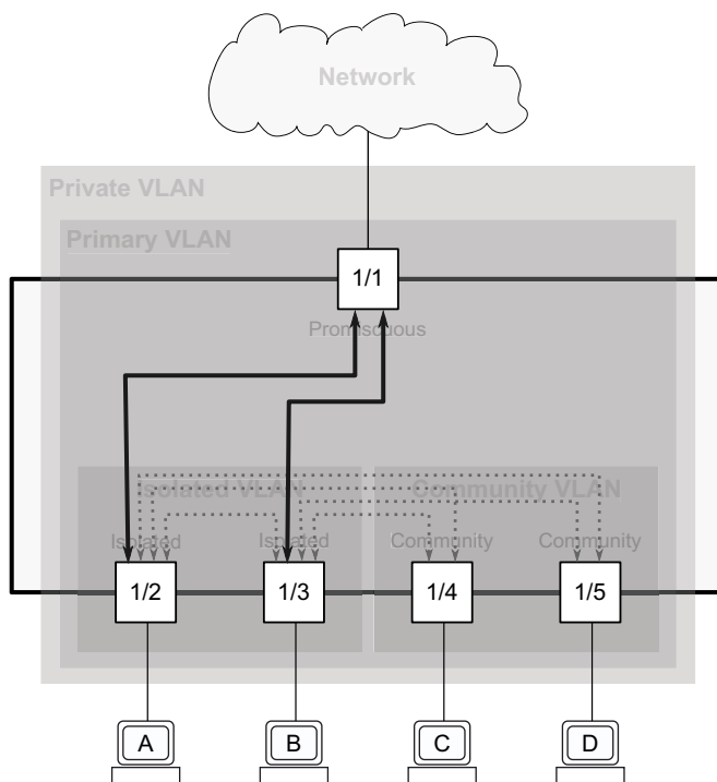
Figure 28: Communication flow of the isolated ports
