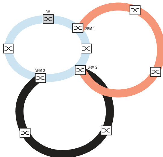
Figure 55: Special case: A Sub Ring Manager device manages 2 Sub Rings (2 instances). The Sub Ring Manager device is capable of managing up to 20 instances.
