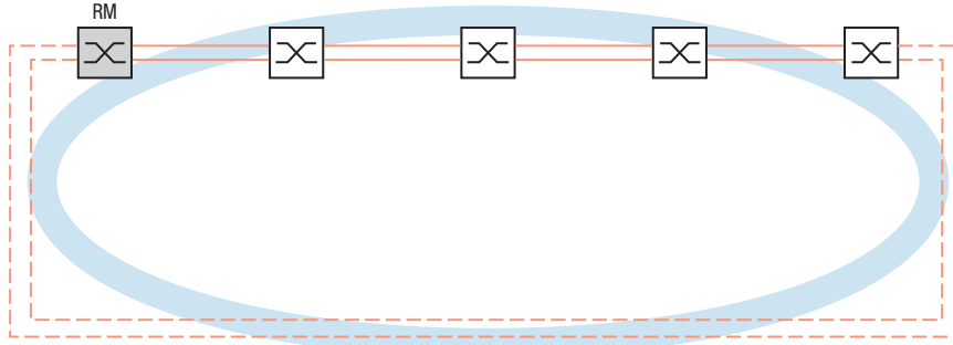
Figure 38: Link Aggregation over the entire MRP Ring.
