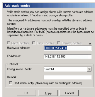
Figure 112: Entries for static addresses
