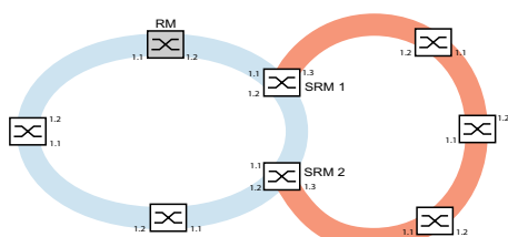
Figure 53: Example of a Sub Ring structure blue ring = Main ring orange ring = Sub Ring SRM = Sub Ring Manager RM = Ring Manager
