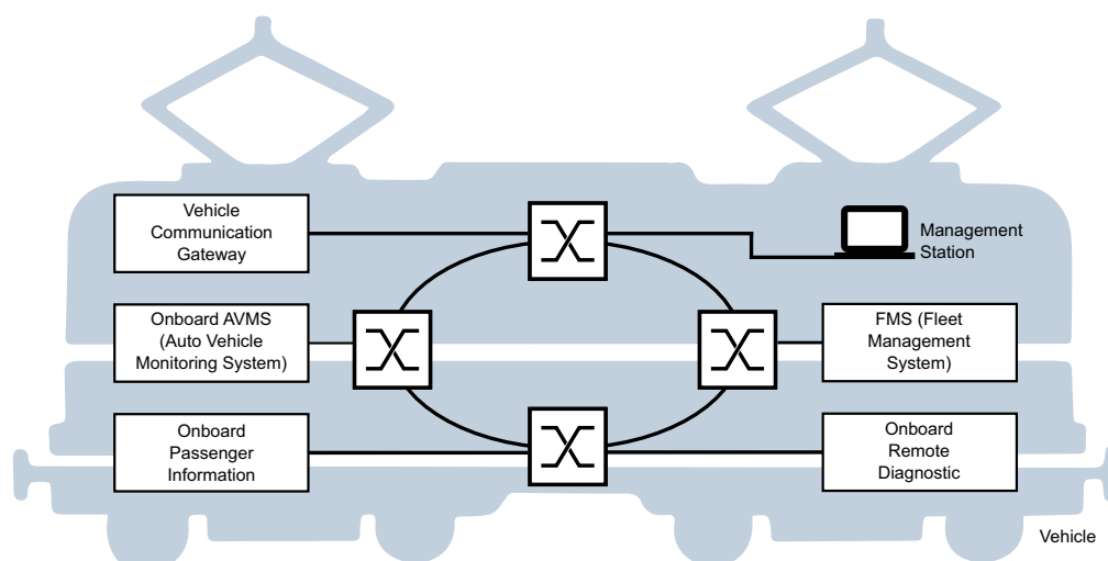
Figure 103: Example for ITxPT Module Inventory
