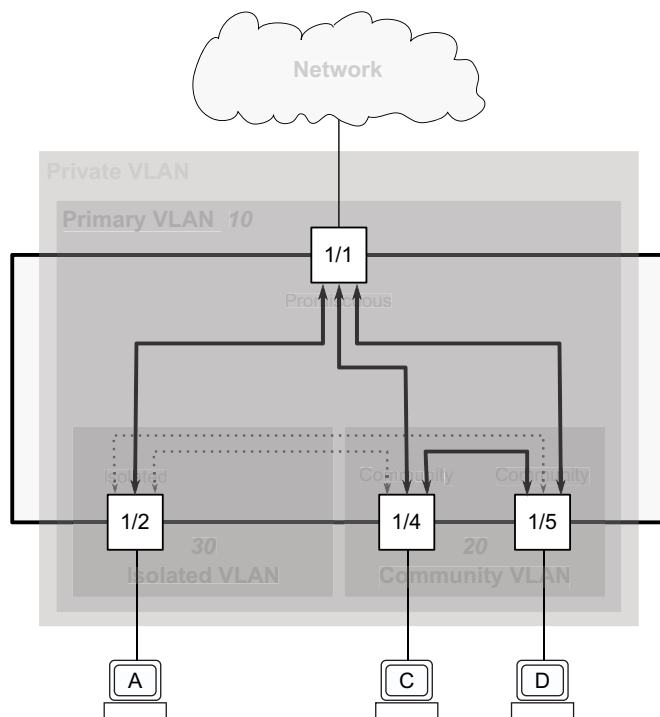
Figure 30: Example of a Private VLAN
