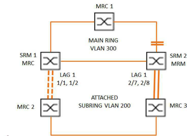
Figure 59: Sub Ring with Link Aggregation
