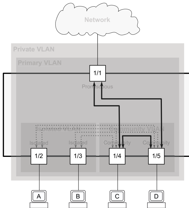
Figure 29: Communication flow of the community ports
