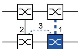
Figure 66: 2-Switch coupling with Control Line, Stand-by device
