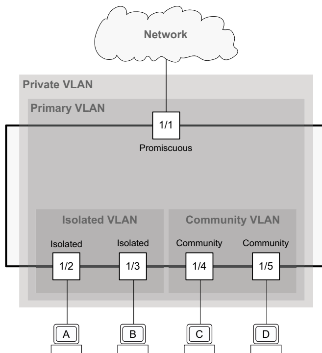
Figure 27: Private VLAN architecture
