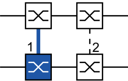
Figure 62: 2-Switch coupling, Primary device 1: Coupling port 2: Partner coupling port
