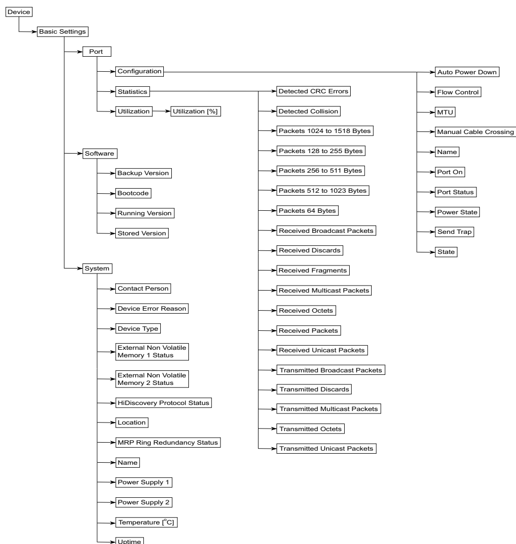
Figure 102: OPC UA information model
