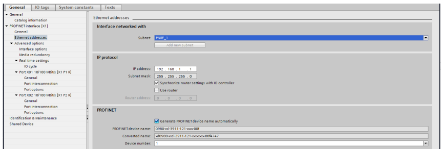
Figure 16: ETHERNET addresses
