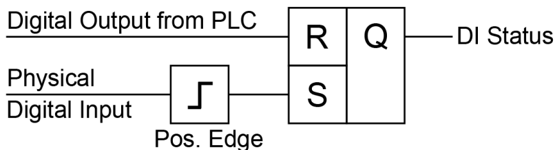
Figure 27: Input latch
