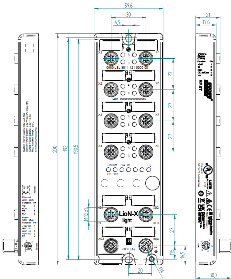
Figure 6: 0980 LSL 3011-121-0006-001
