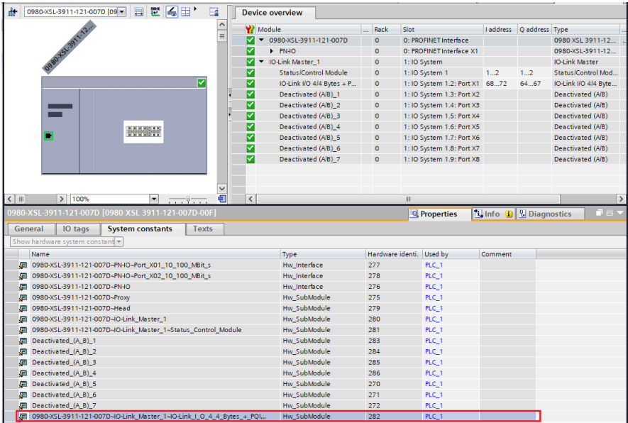
Figure 31: TIA project: Write/Read example with FB50001
