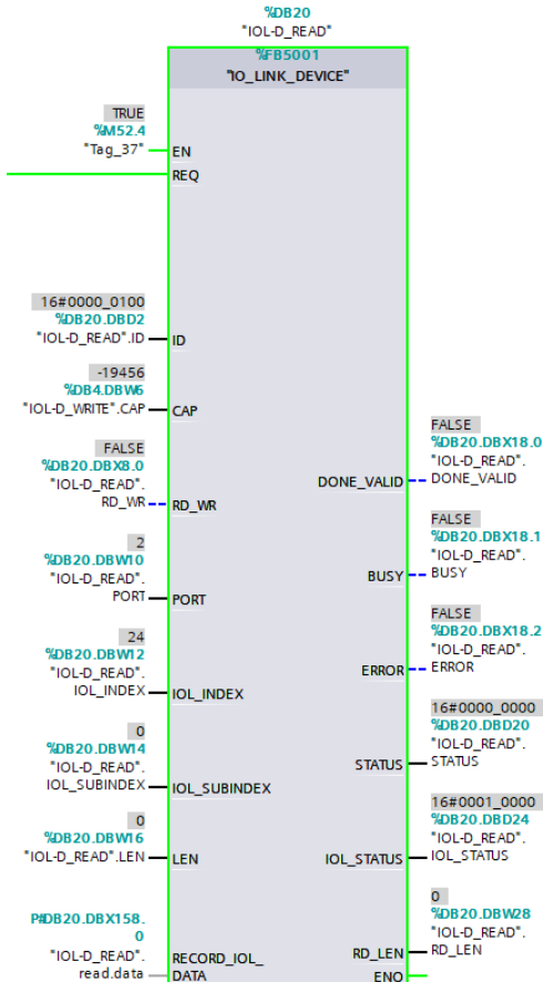
Figure 36: Read example for FB50001
