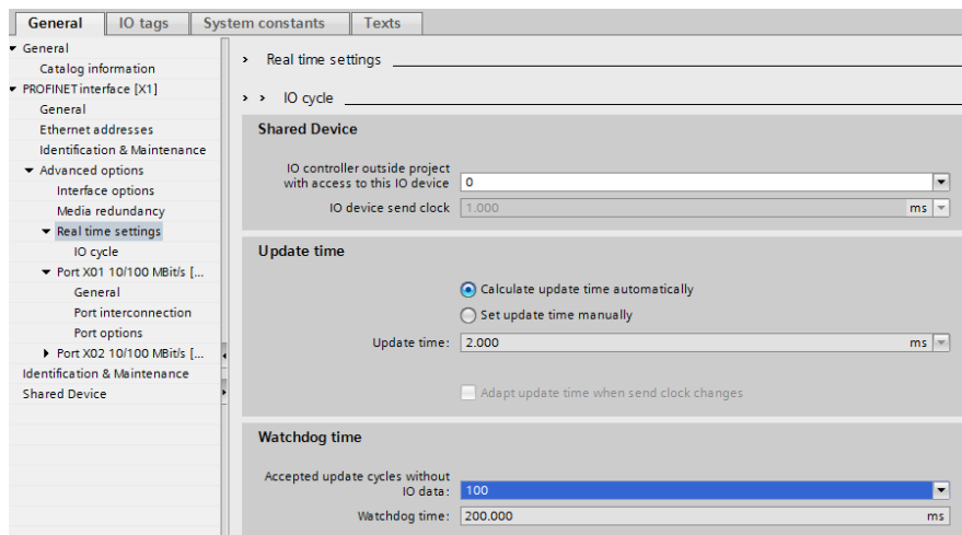
Figure 47: Example of setting up the Watchdog time monitoring in TIA Portal® for using MRP
