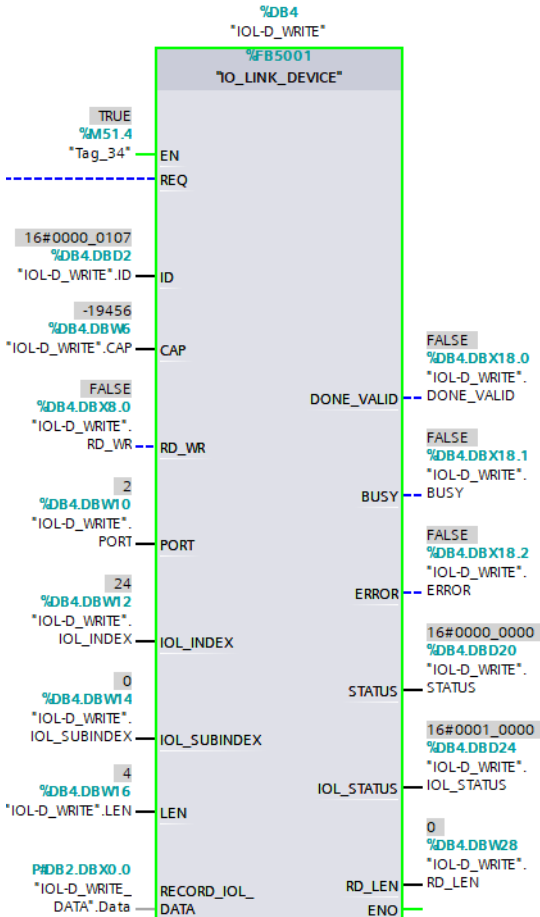
Figure 32: write example for FB50001
