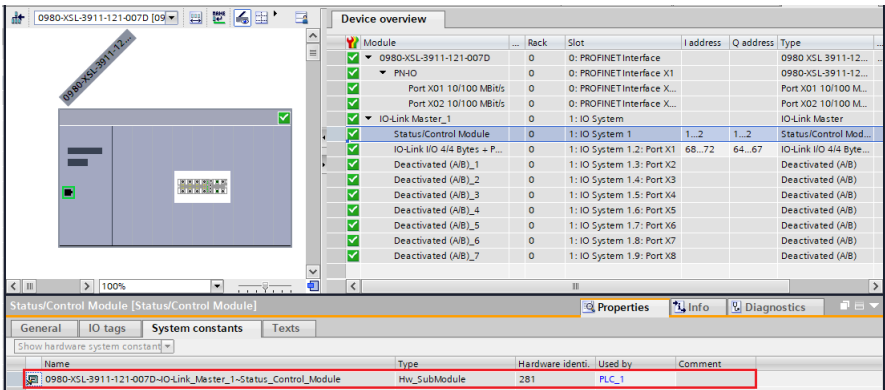
Figure 49: Hardware identifier of the Status/Control Module for RDREC "IO System 1"
