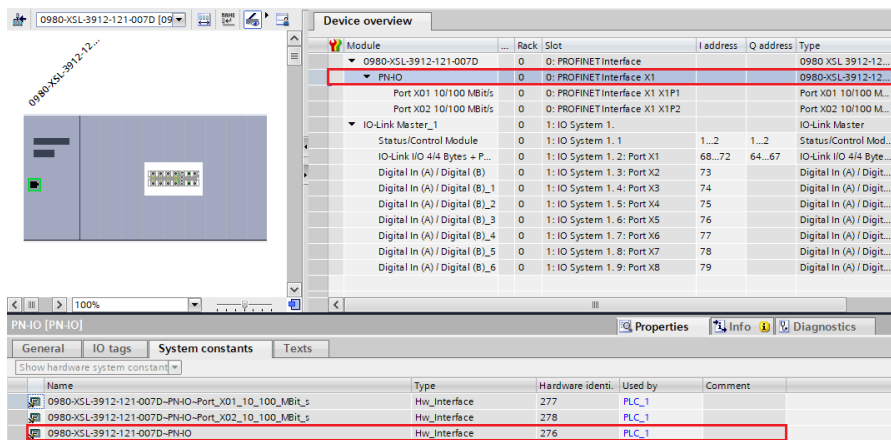
Figure 48: TIA Portal® hardware identifier of PROFINET interface for I&M 0-3 RDREC/WRREC
