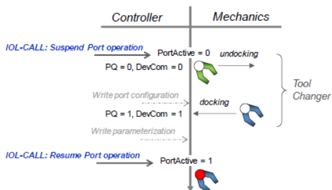
Figure 56: Suspend/Resume Port operation
