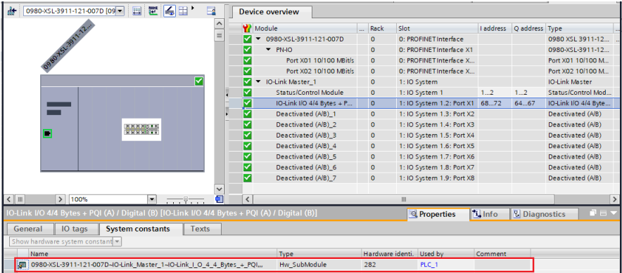
Figure 50: Hardware identifier of the Status/Control module for RDREC "IO System 1.2"
