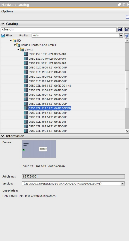
Figure 6: TIA Portal® Hardware catalog
