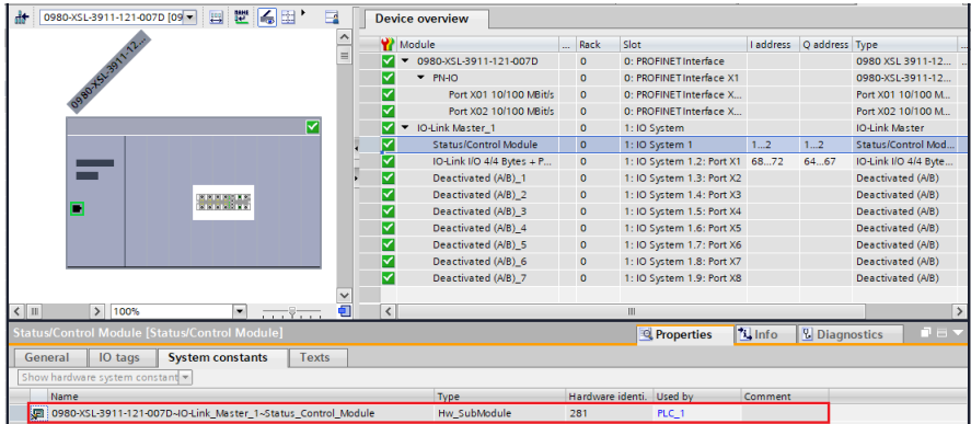
Figure 45: Hardware identifier of the Status/Control Module for RDREC "IO System 1"
