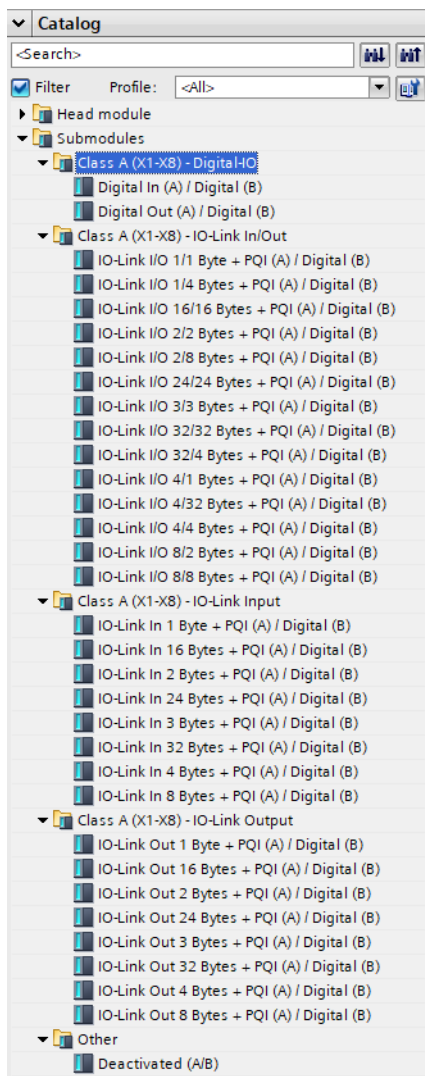
Figure 17: IO-Link channel configuration
