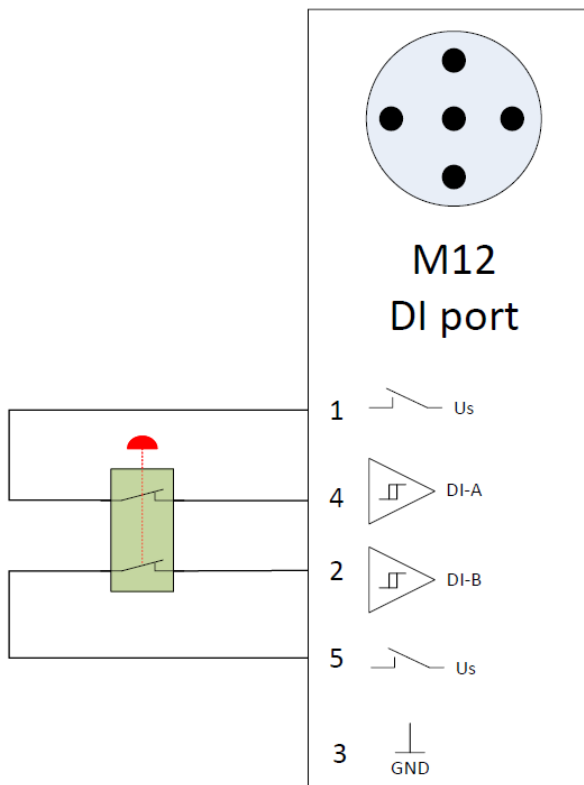
Figure 68: Internal F-DI block diagram
