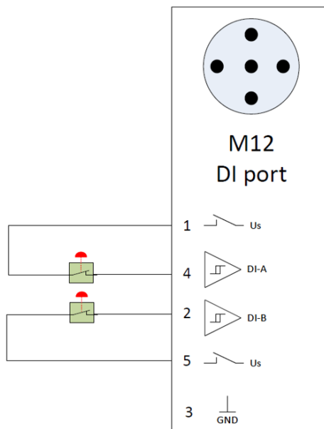
Figure 65: Internal F-DI block diagram
