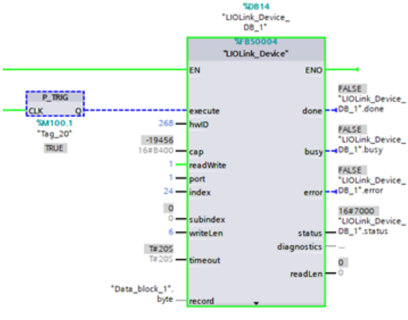
Figure 33: Write example for FB50004
