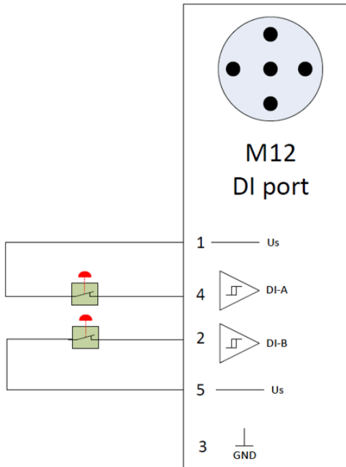
Figure 62: Internal F-DI block diagram
