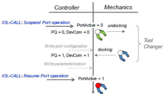
Figure 57: Suspend/Resume Port operation
