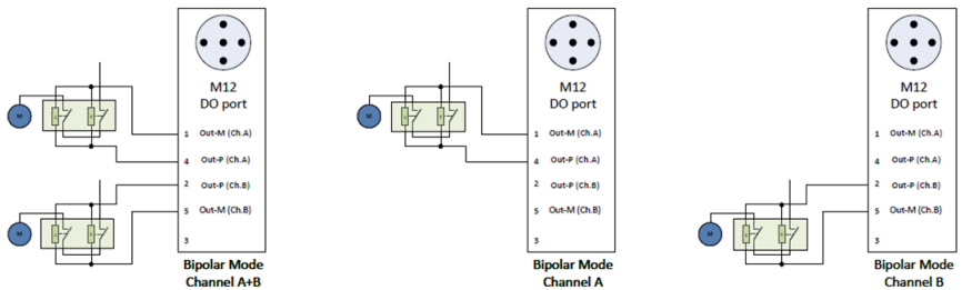
Figure 7: Permitted use cases for the bipolar mode
