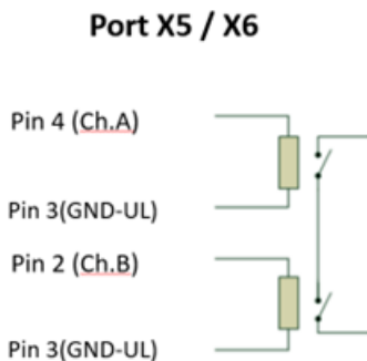
Figure 71: Schematic illustration with two redundant F-DOs
