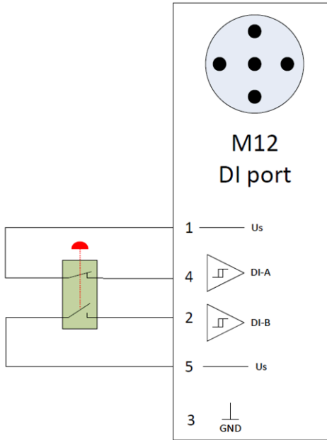
Figure 63: Internal F-DI block diagram
