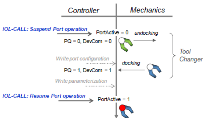
Abb. 57: Suspend/Resume Port operation
