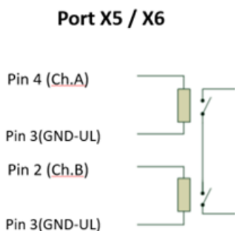
Figure 20: Schematic illustration with two redundant SDOs
