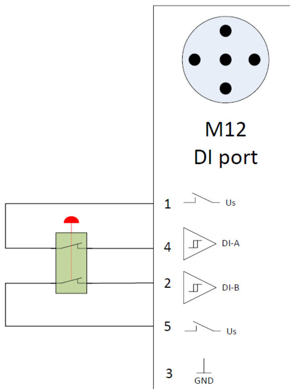
Figure 17: Internal SDI block diagram
