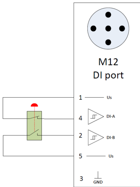
Figure 12: Internal SDI block diagram
