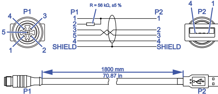
Figure 1: Terminal cable: M12, "A"-coded (male) <-> USB-A
