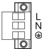
Figure 4: Supply voltage with the characteristic value M9 or K9: 3-pin terminal block with screw locking
