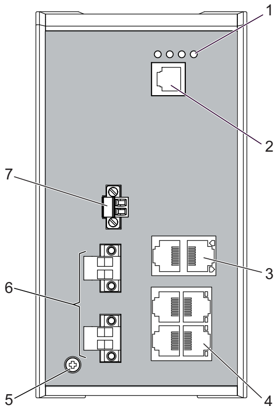
Front view of device variants RSPS.....2T1TT.....
