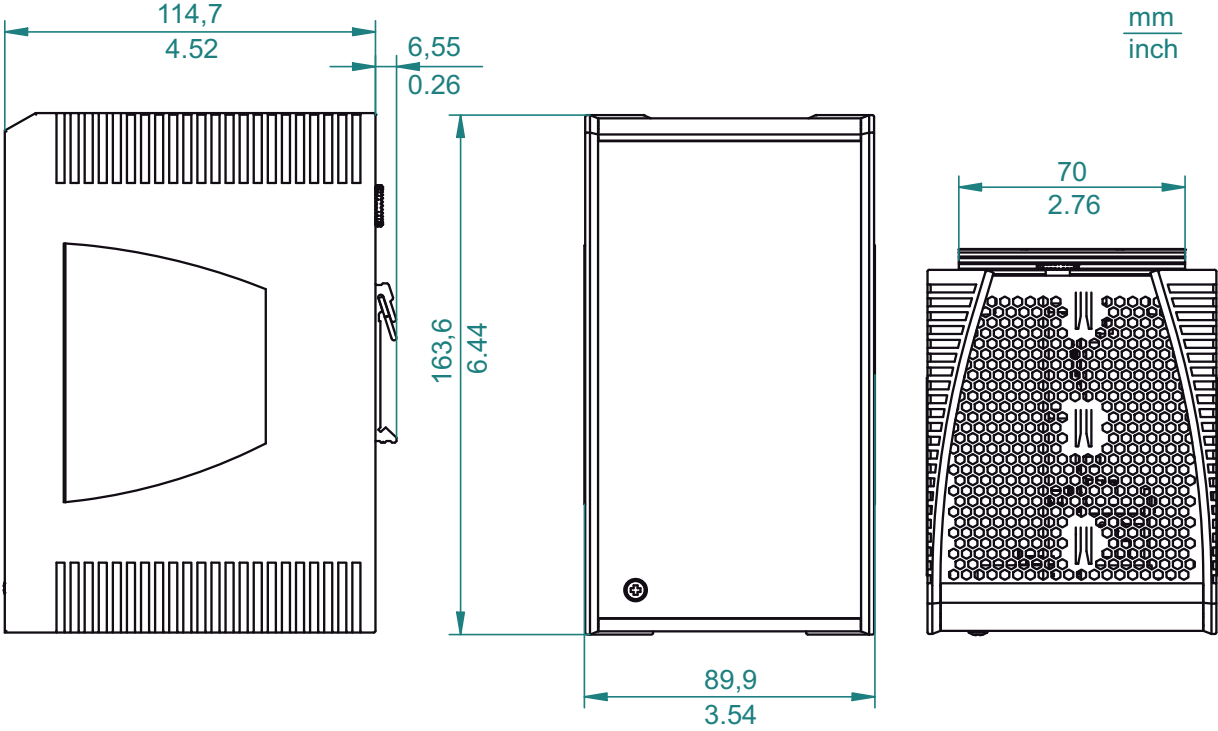
Figure 7: Dimensions
