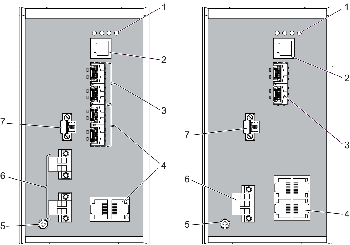
Front view: on the left: Device variants RSPS.....2Z6YT..CC.... on the right: Device variants RSPS.....2Z6TT..M9/K9....
