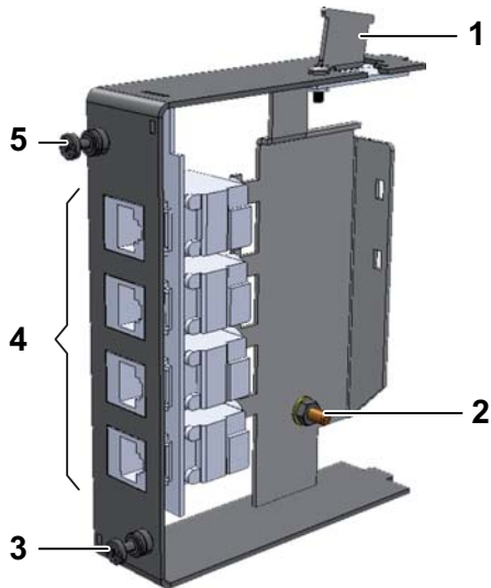
Figure 7: CU single module – components
