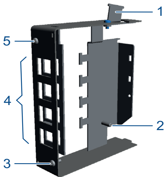
Figure 10: CU module (empty) – components
