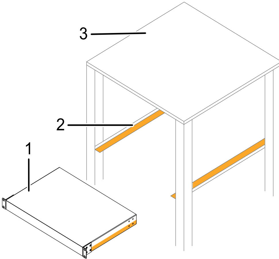
Figure 2: Assembly in a switch cabinet with sliding/mounting rails
