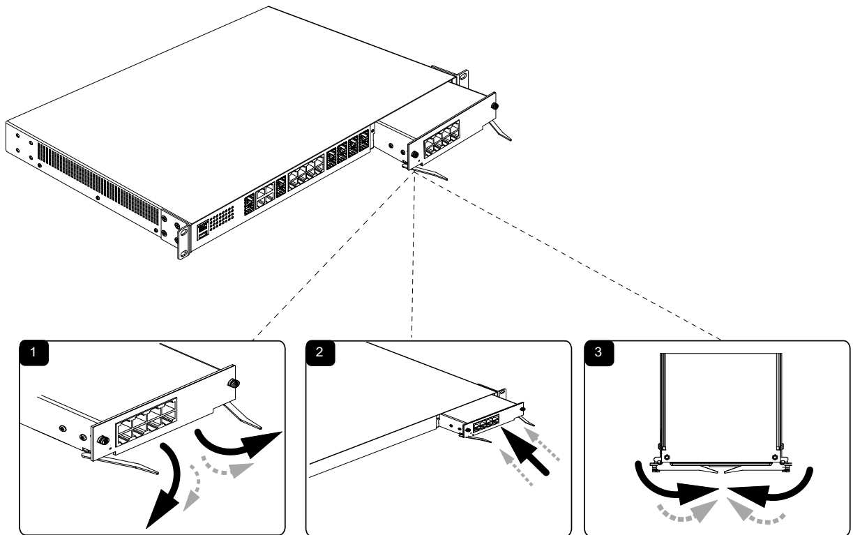
Figure 4: Mounting a media module
