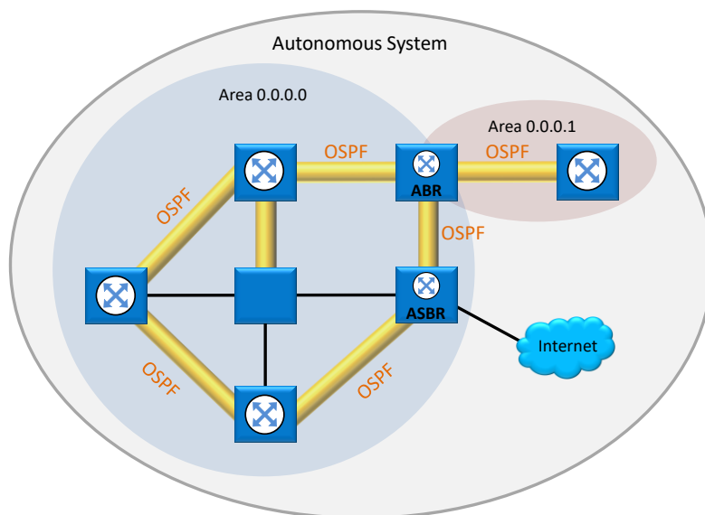
Figure 10 OSPF Example
