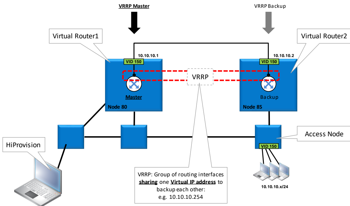
Figure 9 VRRP Example
