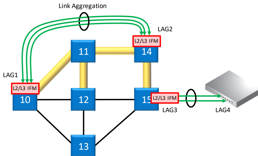
Figure 7 LAG Example
