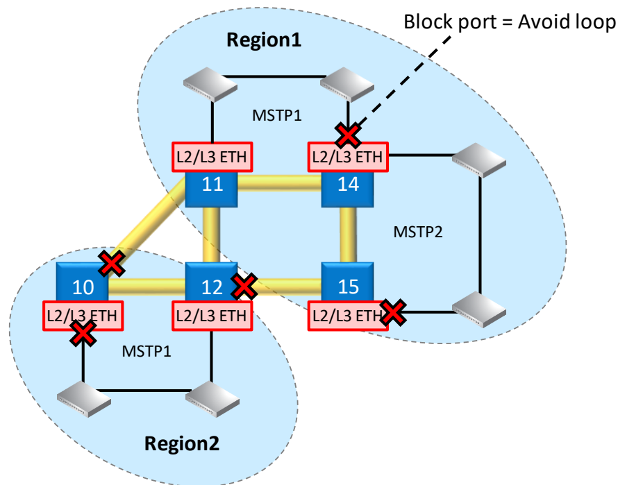
Figure 6 MST Example
