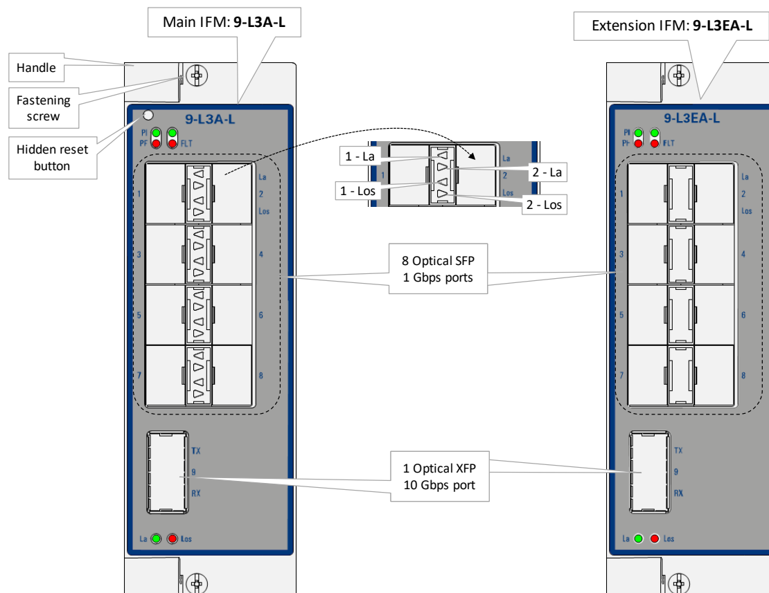
Figure 1 Front Panels: Main L3 Interface Module / Extension L3 Interface Module
