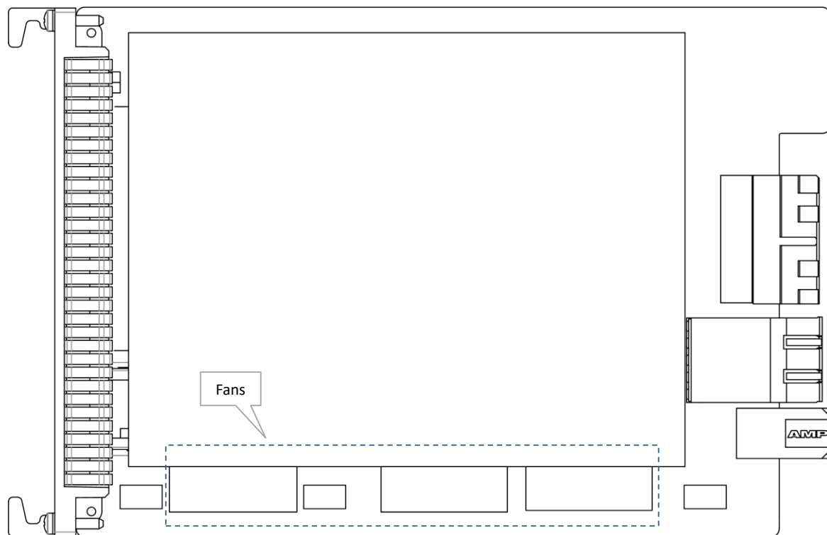
Figure 14 main L3 Interface Module: Side View
