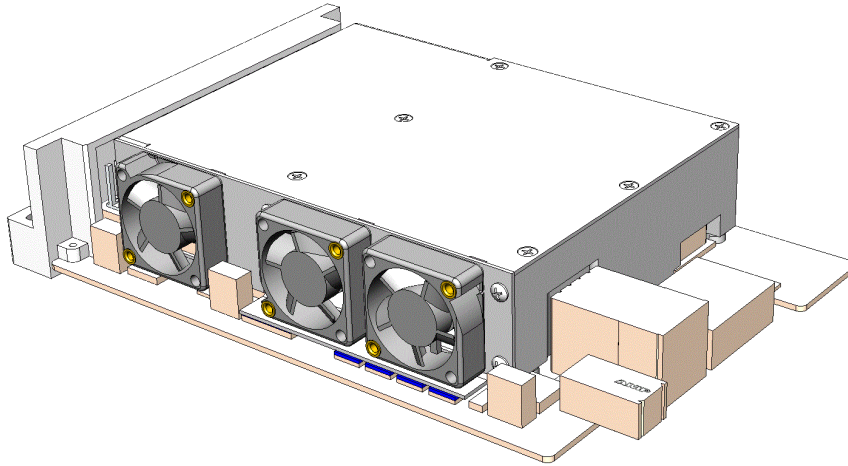
Figure 15 Main L3 Interface Module: 3D View with Fans
