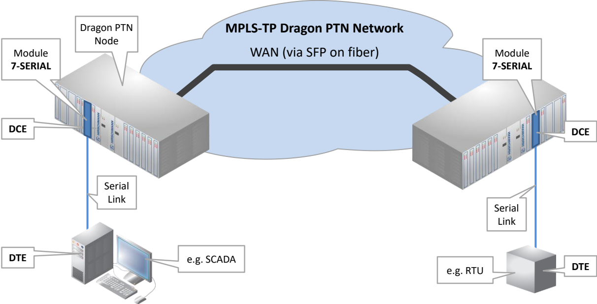
Figure 2 General PTN-7-SERIAL Example
