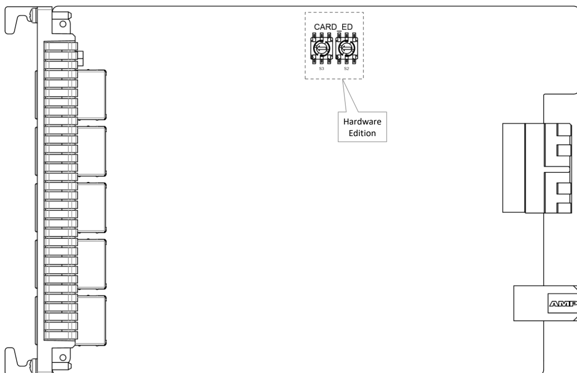
Figure 14 PTN-7-SERIAL: Side View
