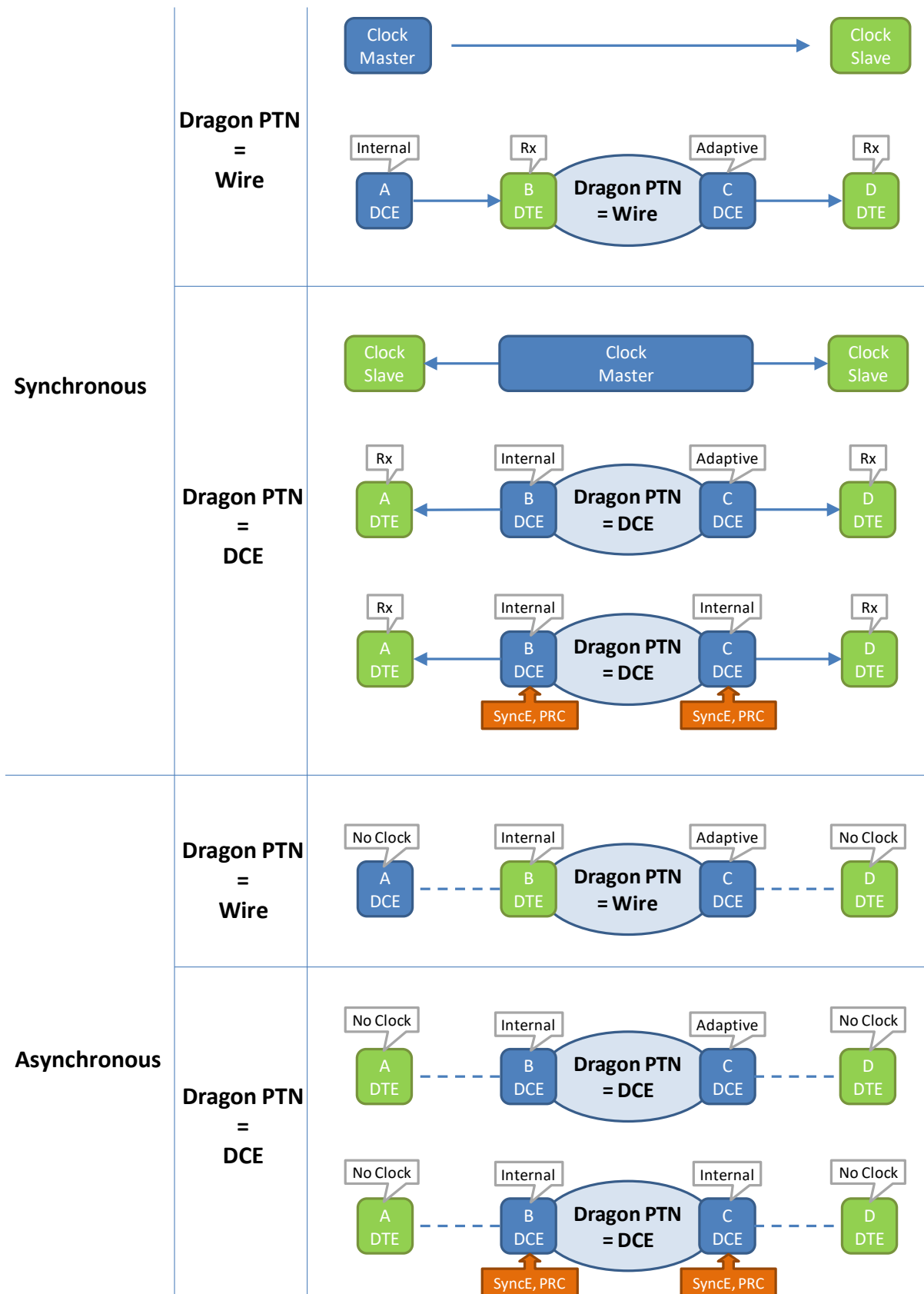
Figure 13 PTN-7-SERIAL Clocking/Synchronization Overview
