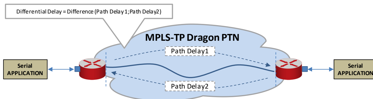
Figure 18 Differential Delay
