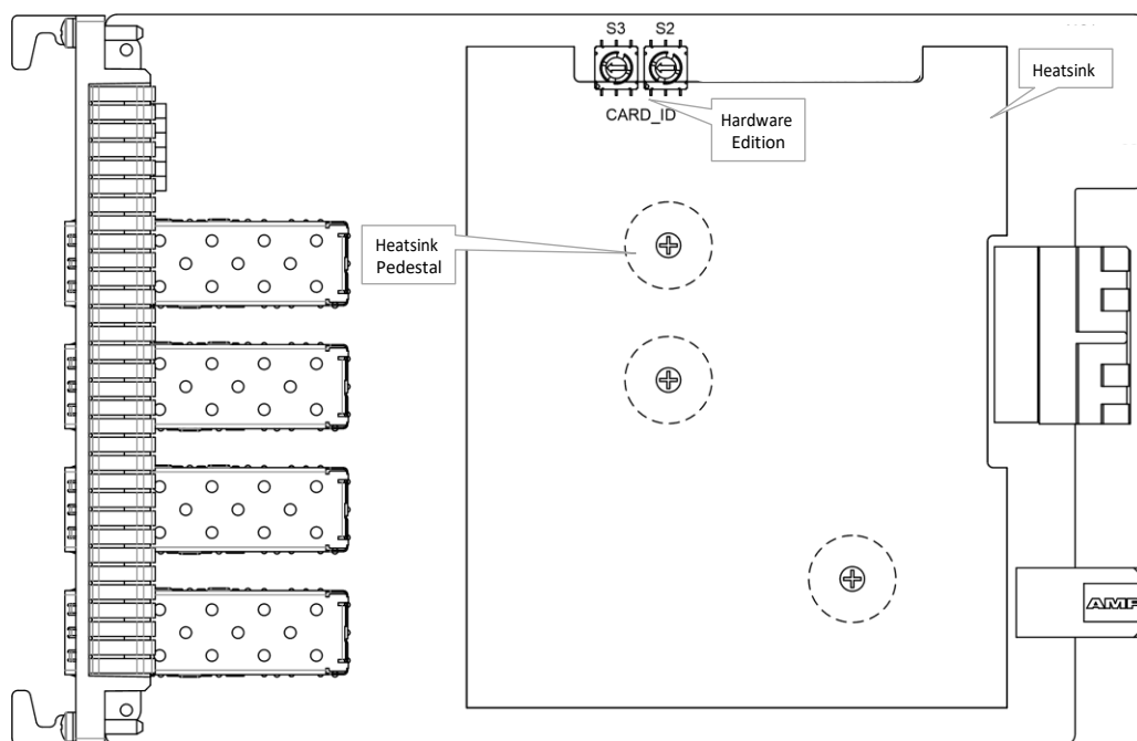
Figure 5 PTN-4-GO-LW: Side View
