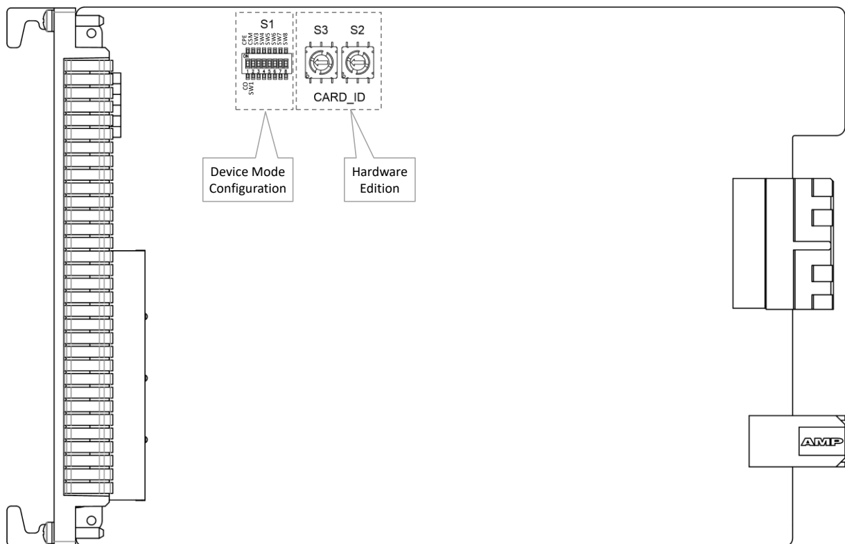
Figure 6 PTN-4-DSL-LW: Side View
