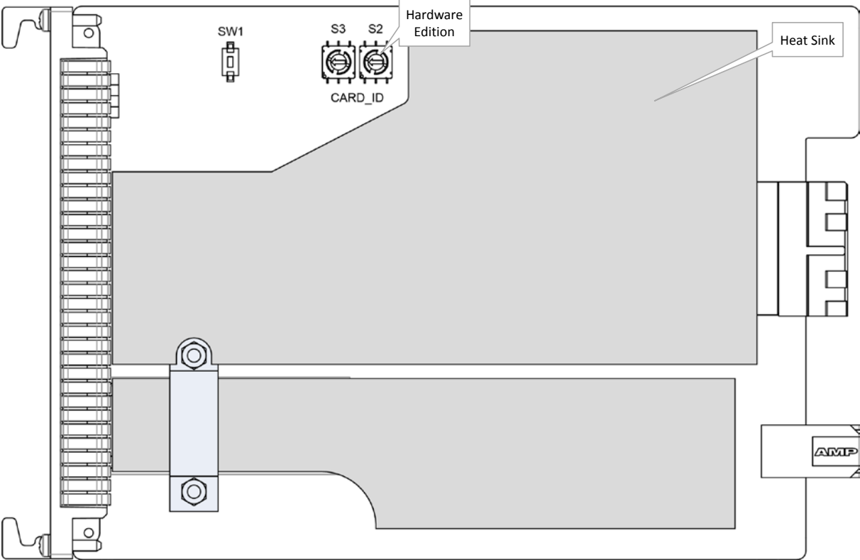
Figure 7 1-10G-LW: Side View
