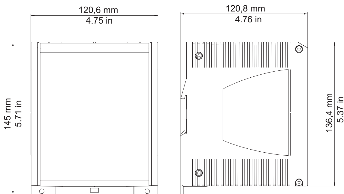
Figure 5: Dimensions of device variants featuring supply voltage with characteristic value W (24 V DC) Note: figure without connections
