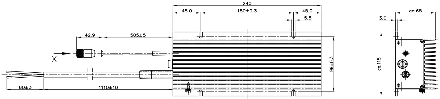
Fig. 1: Dimensions of the PC150/36V/48V-IP67 and PC150/72V/48V-IP67 power supply units
