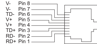
Fig. 6: Pin assignment of a TP/TX interface with PoE, for supply via the the idle wire pairs (spare pairs), RJ45 socket
