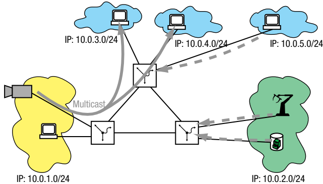
Abb. 116: Multicast-Pruning
