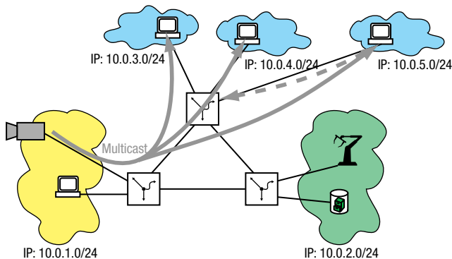
Abb. 117: Multicast-Grafting
