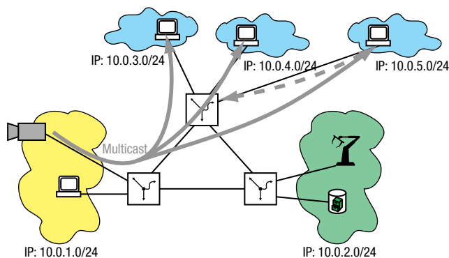
Abb. 113: Multicast-Grafting
