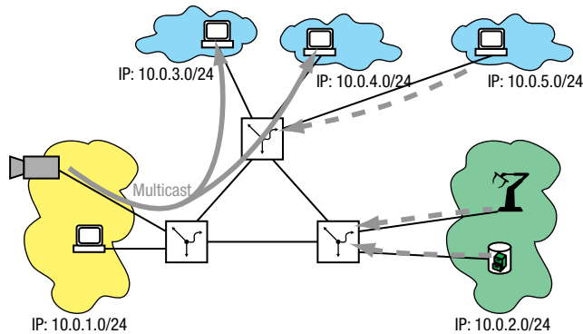
Abb. 112: Multicast-Pruning
