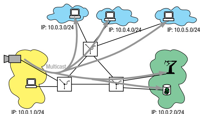
Abb. 111: Multicast Flooding
