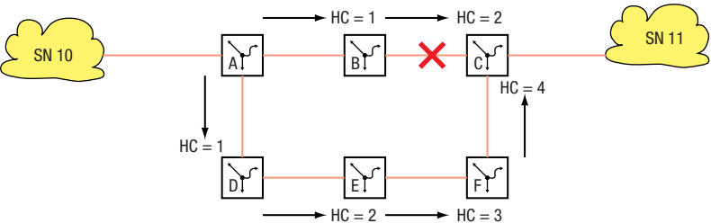
Abb. 100: Hop-Count
