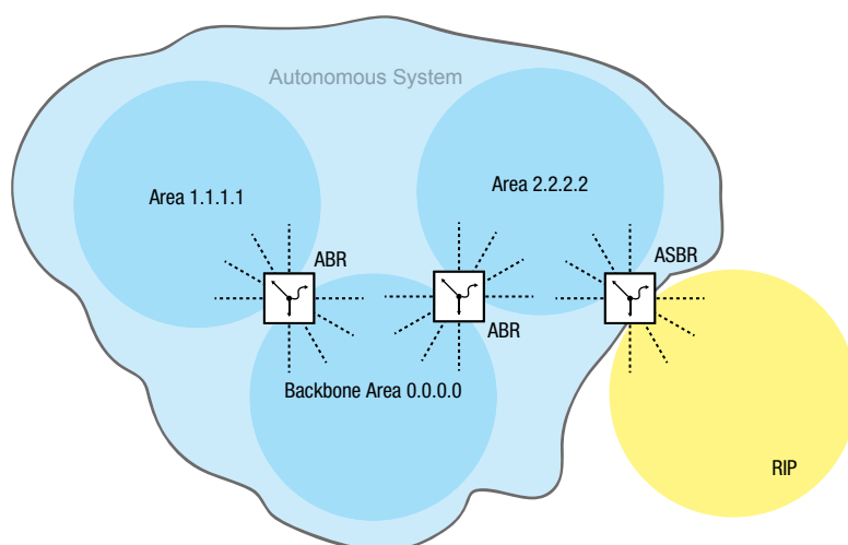
Abb. 102: Autonomes System
