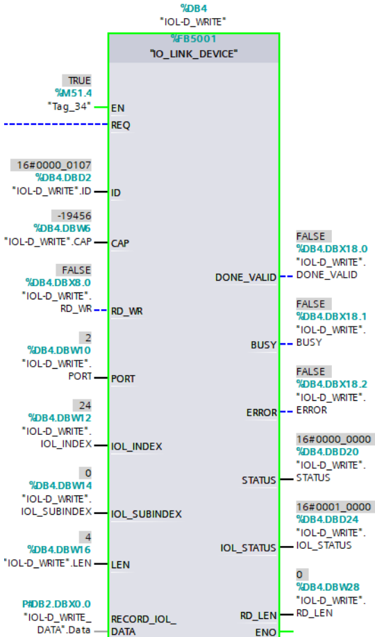
Figure 34: write example for FB50001
