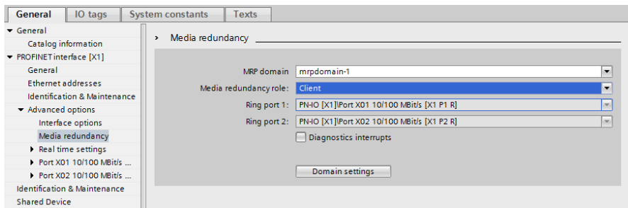
Figure 48: Example of setting up an MRP redundancy client in TIA Portal®
