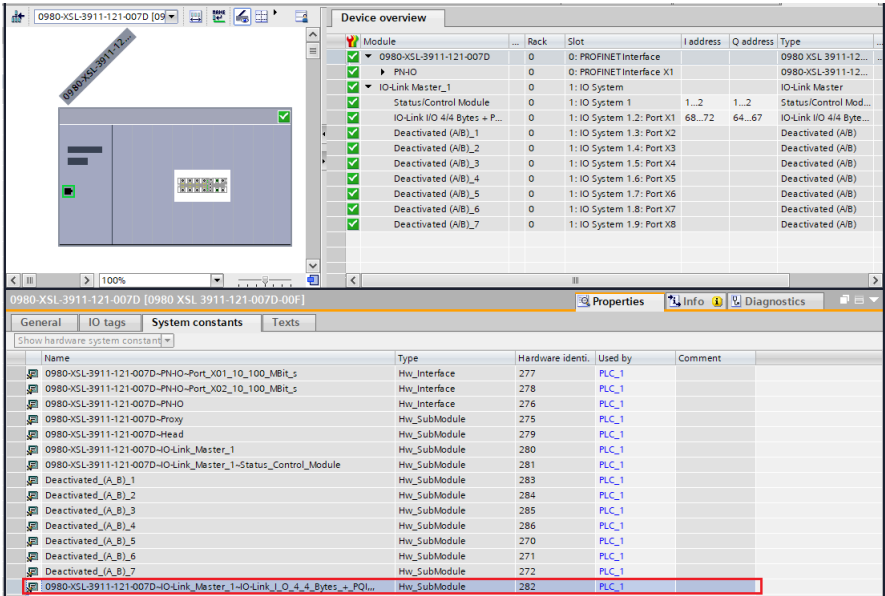
Figure 33: TIA project: Write/Read example with FB50001
