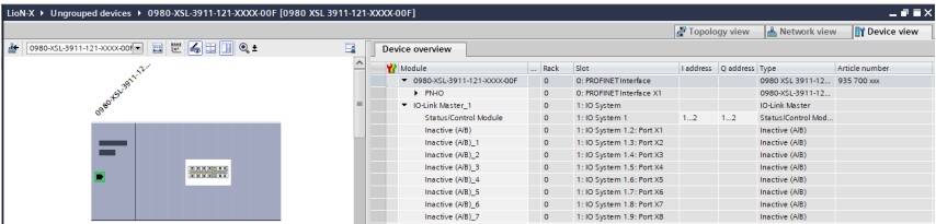
Figure 15: Device configuration
