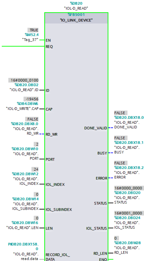
Figure 38: Read example for FB50001
