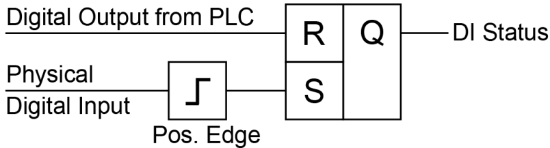
Figure 27: Input latch
