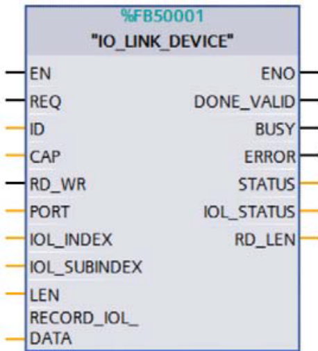
Figure 32: "IO_LINK_DEVICE" FB in STEP 7 V15.1
