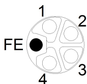
Figure 10: Schematic diagram of the M12 L-coding (socket X04 for Power Out)
