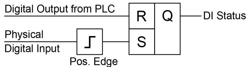
Abb. 12: Input-Latch
