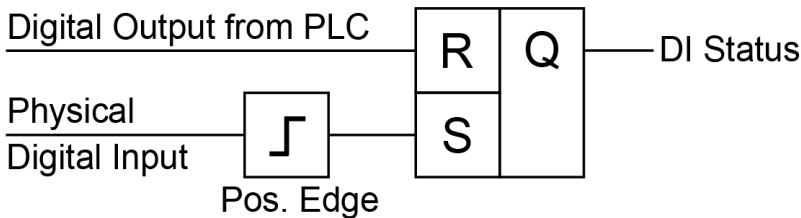
Figure 12: Input latch
