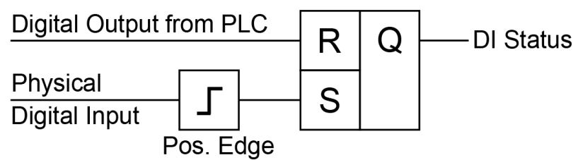
Figure 12: Input latch
