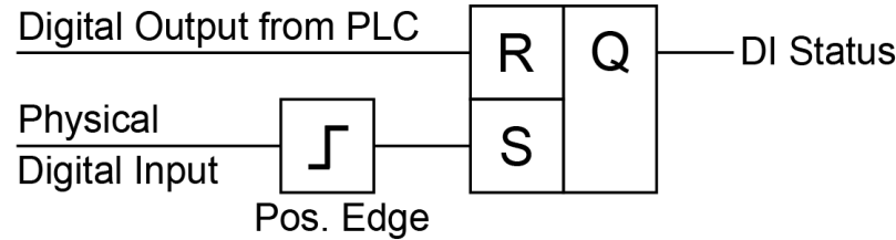
Abb. 12: Input-Latch
